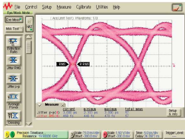
Figure 3-13 N4985A-OA5 ( 2^{31} - 1 ) EYE: <500 fs added rms jitter (5 ps/div)
