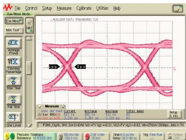
Figure 3-6 N4985A-OA3 ( 2^{31} - 1 ) EYE: <10 ps Tf/Tf (5 ps/div)
