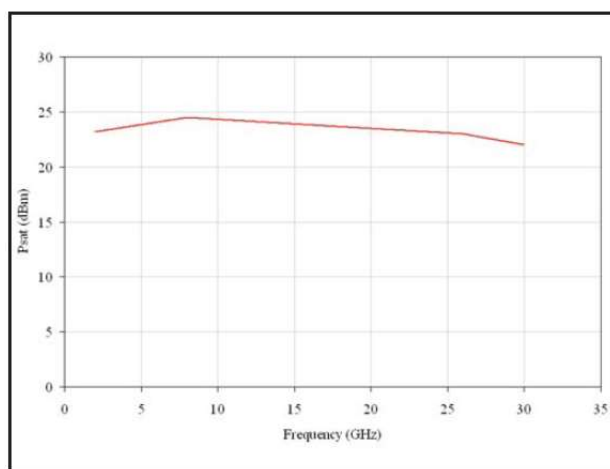
Figure 3-3 Saturated output power (for N4985A-S30)
