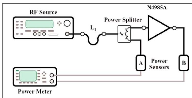
Figure 4-1 Verification setup with a power splitter
