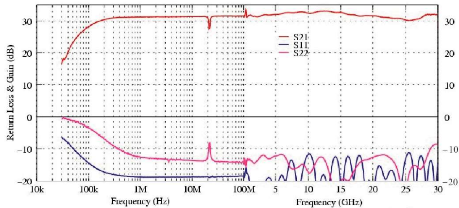
Figure 3-1 Small signal parameters versus frequency (for N4985A-S30)
