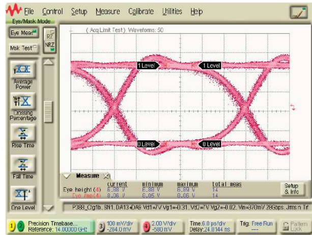
Figure 3-4 N4985A-OA3 ( 2^{31} - 1 ) EYE: >7 V output (1.5 V/div)
