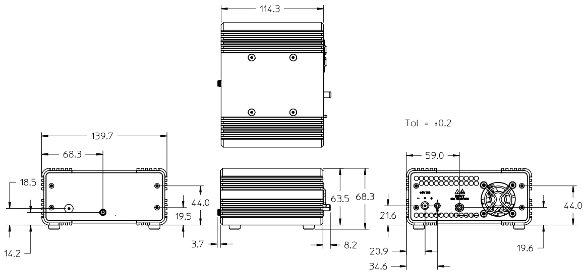
Figure 3-25 Mechanical dimensions of the N4985A-P15/N4985A-P25 amplifier
