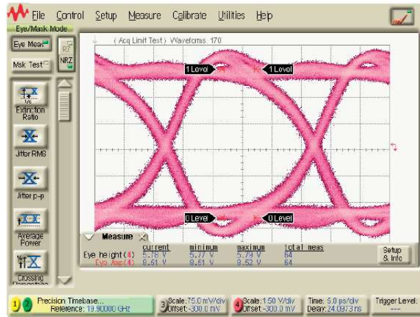
Figure 3-12 N4985A-OA5 ( 2^{31} - 1 ) EYE: >7 V output (1.5 V/div)
