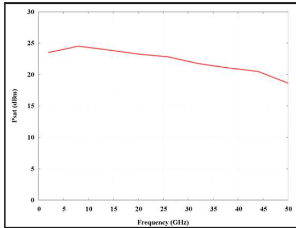
Figure 3-10 Saturated output power (for N4985A-S50)
