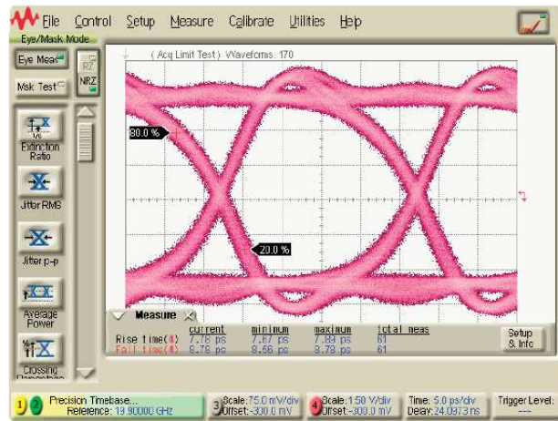
Figure 3-14 N4985A-OA5 ( 2^{31} - 1 ) EYE: <10 ps Tf/Tf (5 ps/div)
