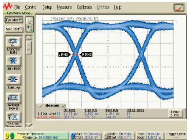
Figure 3-15 N4985A-OA5 ( 2^{31} - 1 ) EYE: Input signal from PRBS generator
