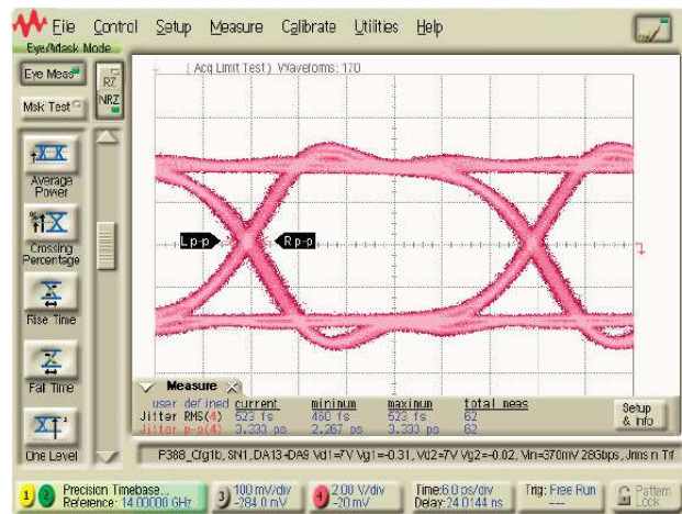
Figure 3-5 N4985A-OA3 ( 2^{31} - 1 ) EYE: <500 fs added rms jitter (5 ps/div)
