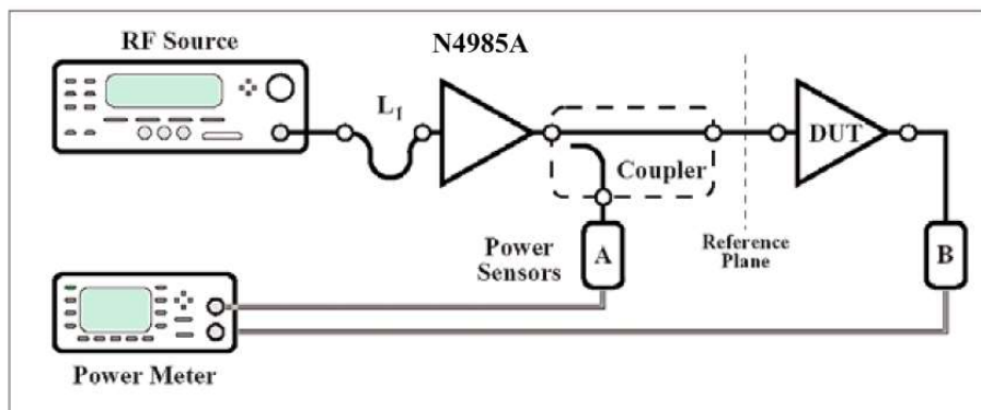
Figure 4-3 Example of an amplified RF power measurement system
