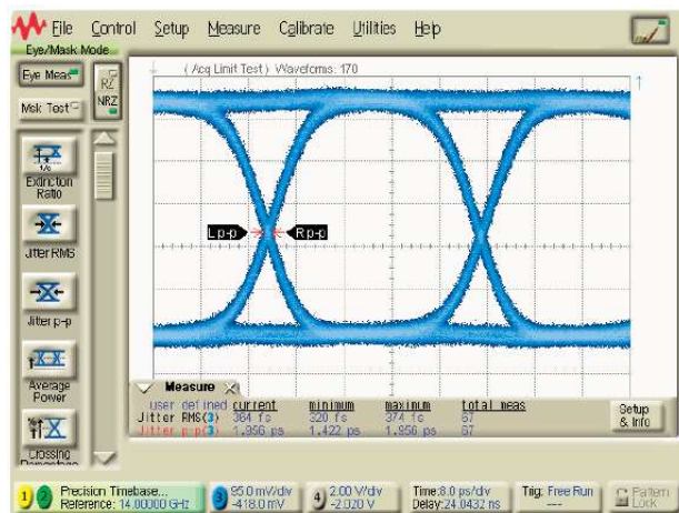
Figure 3-7 N4985A-OA3 ( 2^{31} - 1 ) EYE: Input signal from PRBS generator
