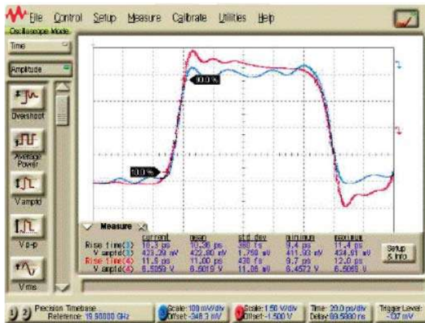
Figure 3-11 Input pulse = Ch3, 420 m Vppk, 10.4 pS rise time, Output pulse = Ch4, 6.5 Vppk, 11.0 pS rise time (for N4985A-S50)
