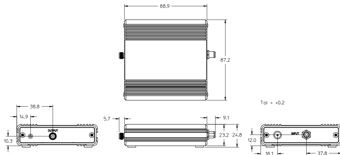
Figure 3-24 Mechanical dimensions of the N4985A-S30/N4985A-S50 amplifier
