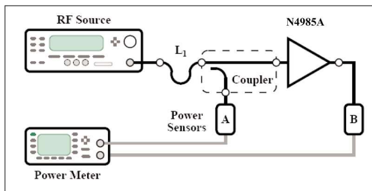
Figure 4-2 Verification setup with a calibrated coupler
