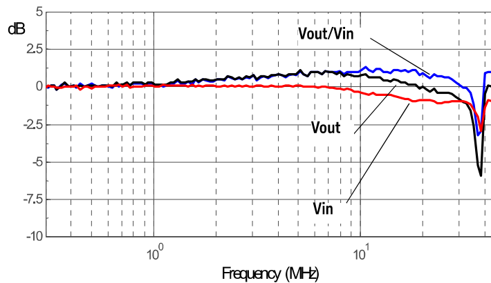
Figure 5 Graph of \text{dB}(\text{Vin}) , \text{dB}(\text{Vout}) + 40\text{dB} , and \text{dB}(\text{Vout}/\text{Vin}) + 40\text{dB} frequency response, 100:1 attenuation
