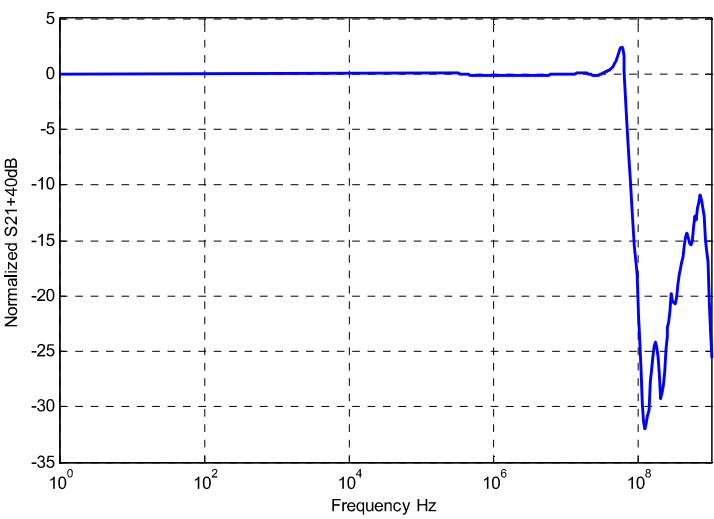
Figure 11 Graph of dB (S21) + 40 dB frequency response, 100:1 attenuation
