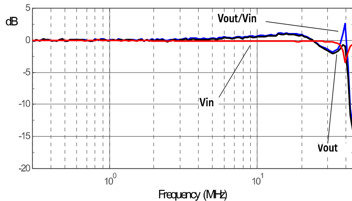
Figure 4 Graph of \text{dB}(\text{Vin}) , \text{dB}(\text{Vout}) + 20\text{dB} , and \text{dB}(\text{Vout}/\text{Vin}) + 20\text{dB} frequency response, 10:1 attenuation
