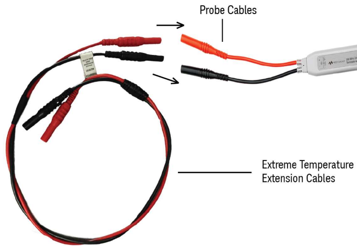
Figure 17 Connecting the Extreme Temperature Differential Extension Cables
