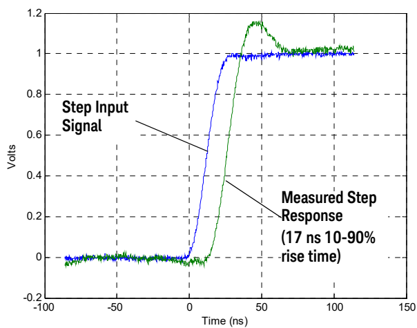
Figure 2 Graph of normalized step response (50Ω, 16.5 ns rising edge step generator), 17 ns normalized rising edge (10-90%), 10:1 attenuation
