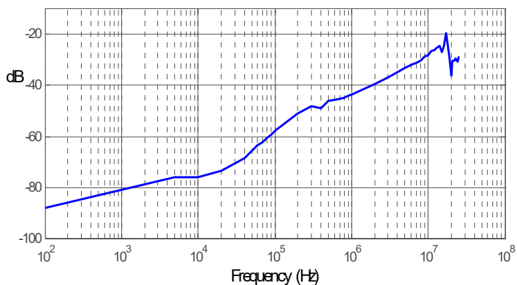
Figure 6 Graph of \text{dB} (V_{\text{out}}/V_{\text{in}}) + 20\text{dB} frequency response when inputs driven in common mode (common mode rejection), 10:1 attenuation
