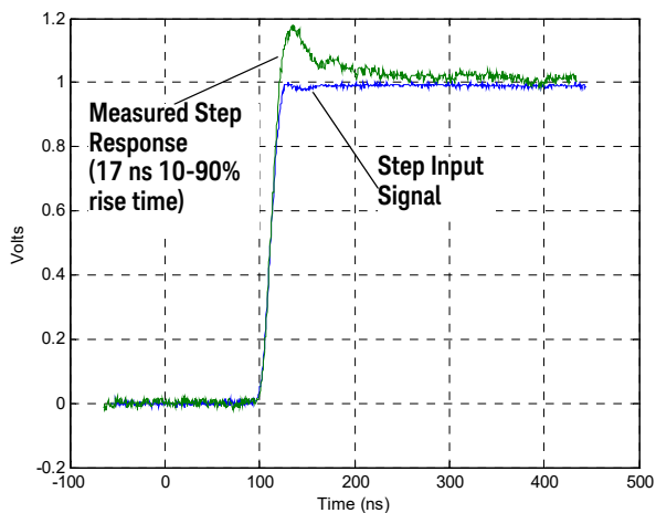
Figure 3 Graph of normalized step response (50Ω, 17 ns rising edge step generator), 17 ns normalized rising edge (10-90%), 100:1 attenuation
