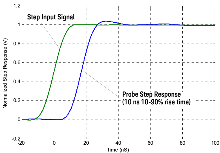
Figure 10 Graph of normalized step response (50 \Omega , 10 ns rising edge step generator), 10 ns normalized rising edge (10-90%), 1000:1 attenuation
