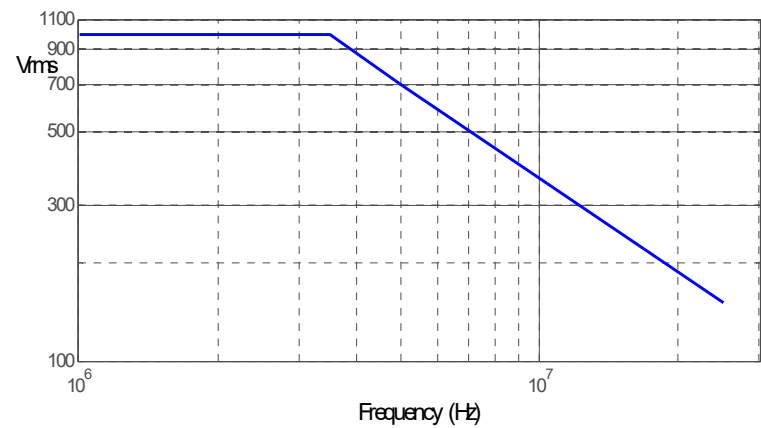
Figure 8 Typical derating plot of the absolute maximum input voltage in common mode
