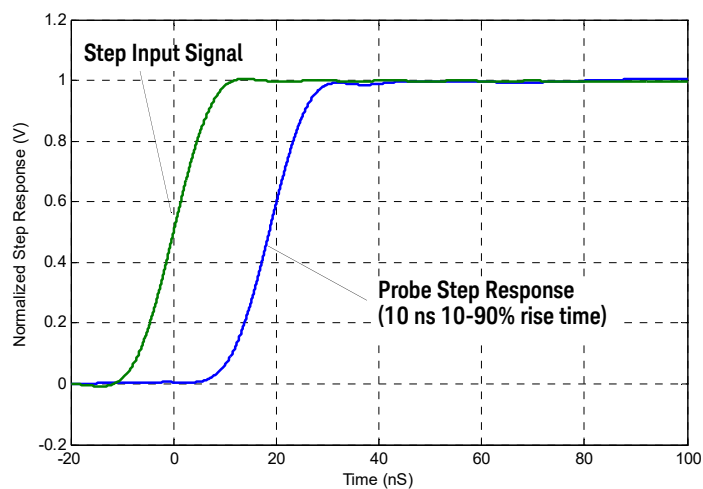
Figure 9 Graph of normalized step response (50 \Omega , 10 ns rising edge step generator), 10 ns normalized rising edge (10-90%), 100:1 attenuation
