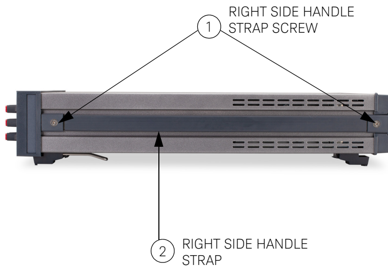
Figure C-1 3458A right side
