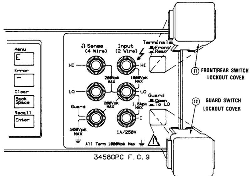
Figure C-9 Switch covers installation
