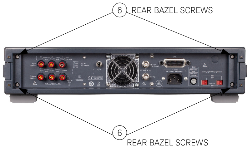
Figure C-4 3458A rear view
