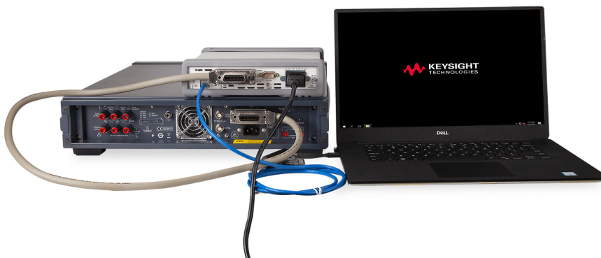
Figure 1-4 Typical GPIB connections
