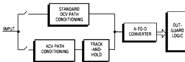
Figure E-3 The 3458A multimeter (RoHS Compliance) provides two different digitizing paths, the standard DCV path and a track-and-hold path.
