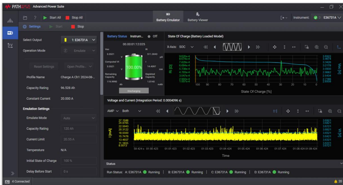
Figure 6. PW9253A connected to a two-quadrant power supply
