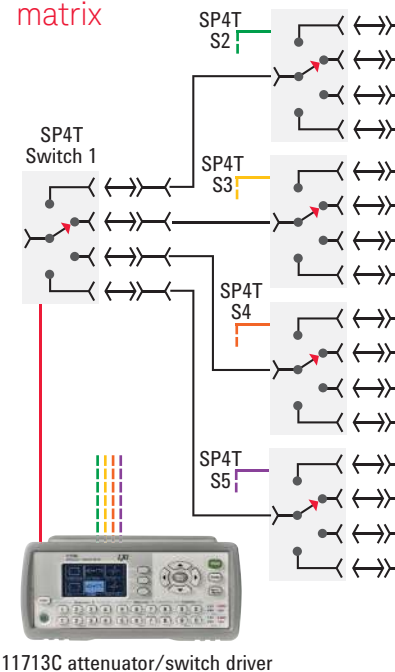
11713C attenuator/switch driver
