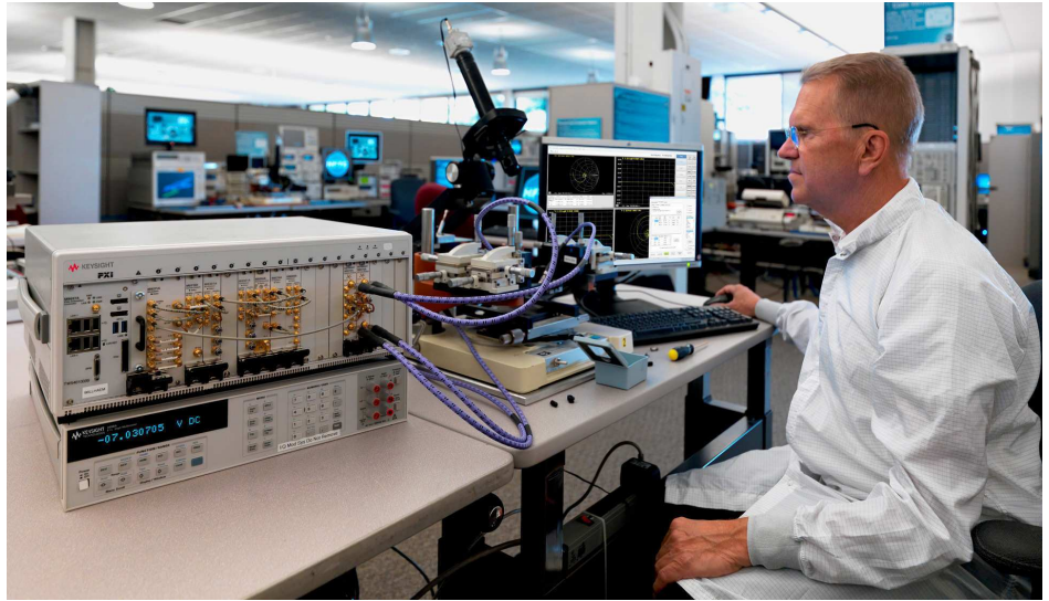
Figure 1. Using Keysight's M937xA PXIe vector network analyzer, M9381A PXIe vector signal generator and M9391A PXIe vector signal analyzer with measurement application software for power amplifier test.
