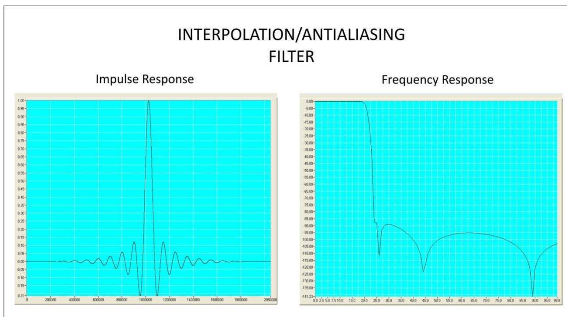
Figure 18: Interpolation/Antialiasing filter
