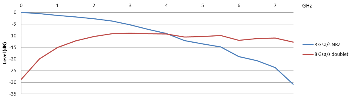
Frequency Response, includes sin x/x roll-off (typ.)
