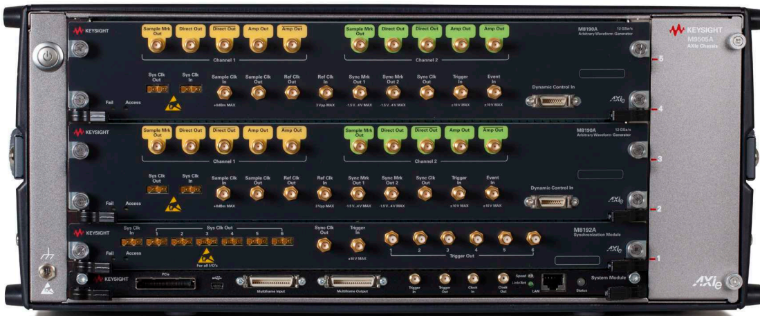
Five slot AXle chassis with two M8190A AWG; can contain an embedded controller.
