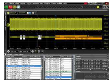
Trigger on and decode SATA serial packets
