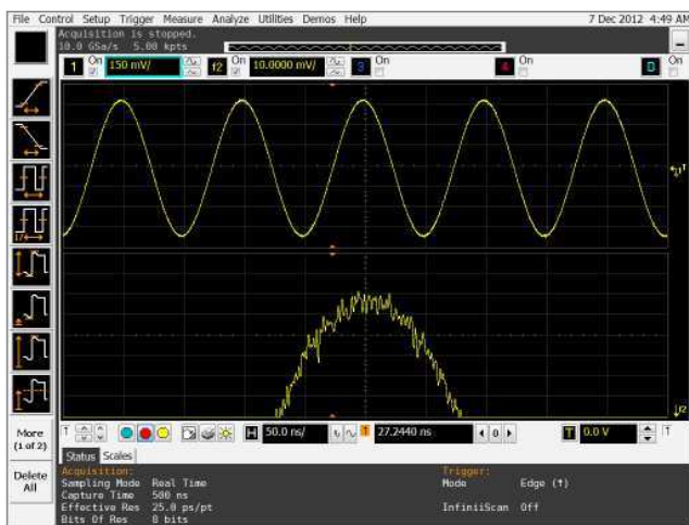
Zoom on top of clean sin wave shows more noise with 8-bit scope
