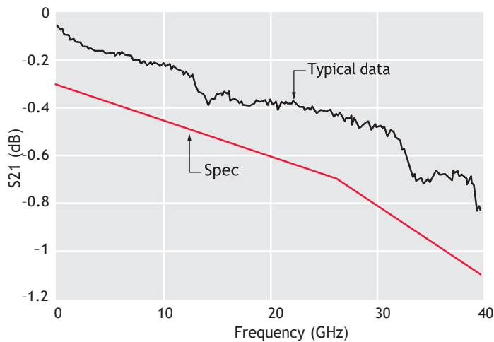
Figure 9. 87104/6D insertion loss versus frequency
