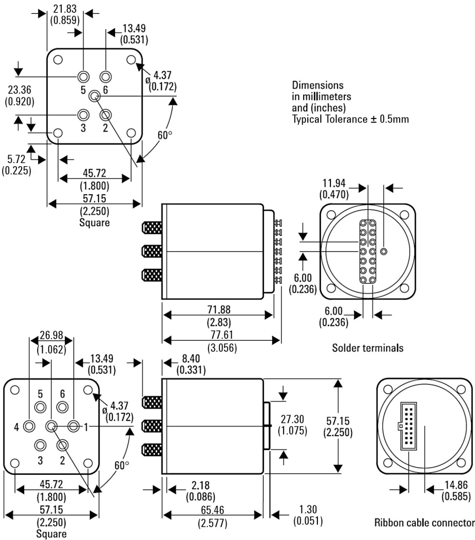
Figure 11. Mechanical dimensions
