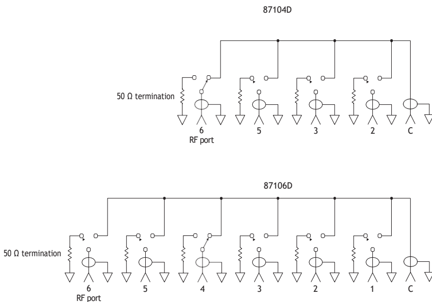
Figure 2. Keysight 87104D and 87106D simplified schematics
