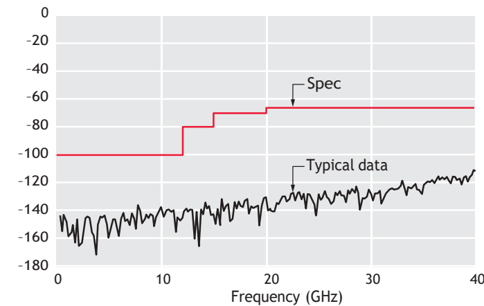
Figure 10. 87104/6D isolation loss versus frequency
