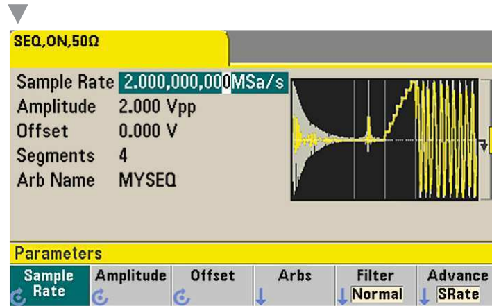
Waveform generator display with downloaded waveform.
