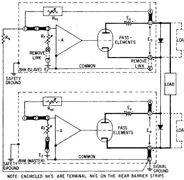
FIG. 3-21 "MASTER-SLAVE" SERIES CONNECTION (MASTER UNIT CONTROL OF OUTPUT).
