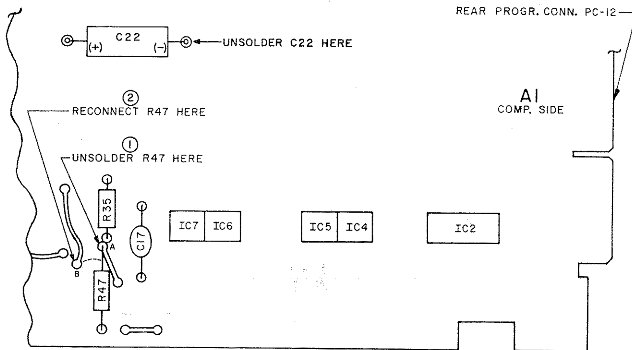
FIG. 3-27 LOCATION OF OVERVOLTAGE SENSING LEAD DISCONNECT.
