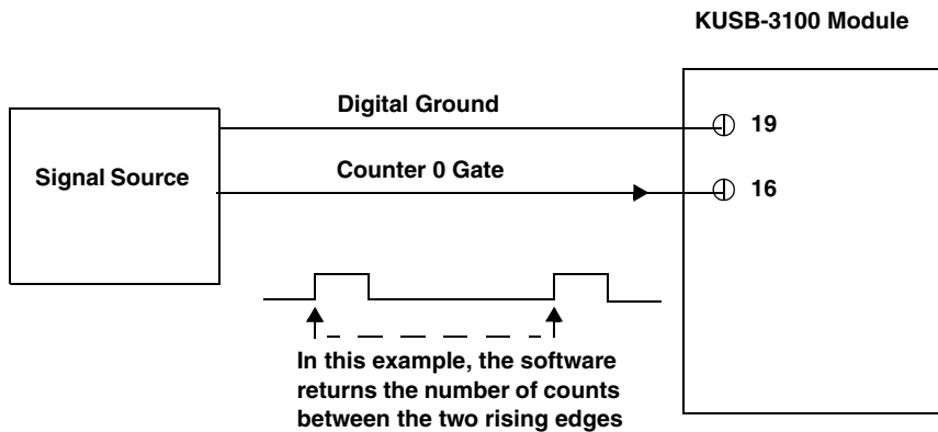
Figure 11: Connecting Counter/Timer Signals for an Edge-to-Edge Measurement Operation
