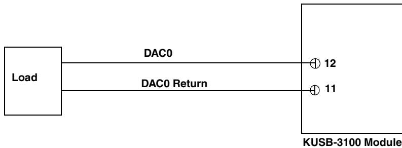
Figure 5: Connecting Analog Outputs to a Screw Terminal Panel
