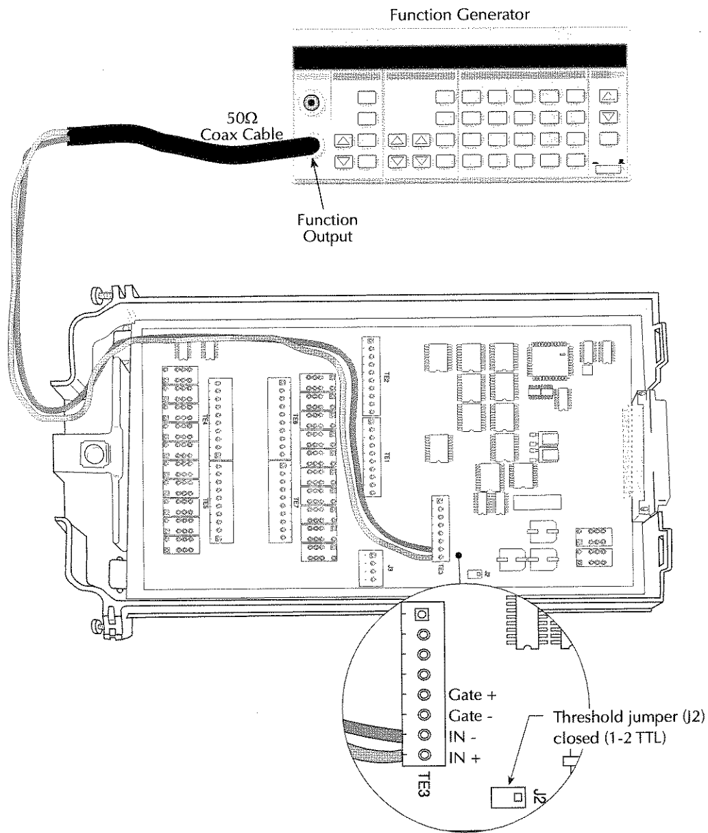
Figure 25 Verification—Totalizer connections
