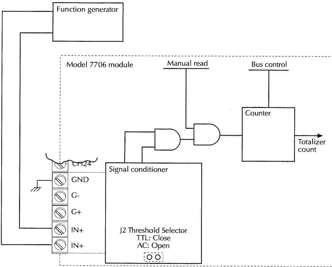
Figure 18 Totalizer
