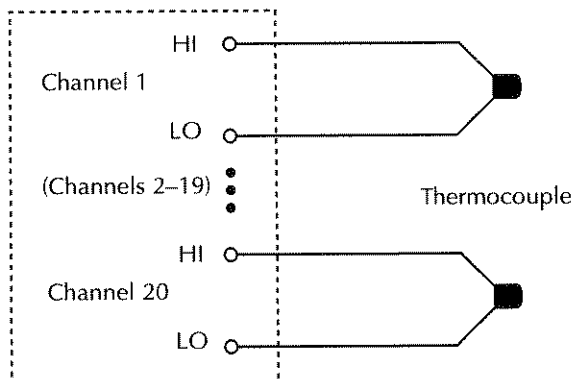
Figure 5 Thermocouple connections
