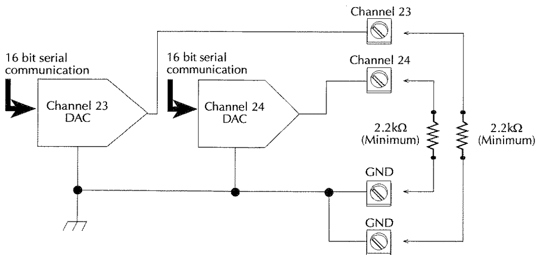
Figure 16 Sample analog connection schematic
