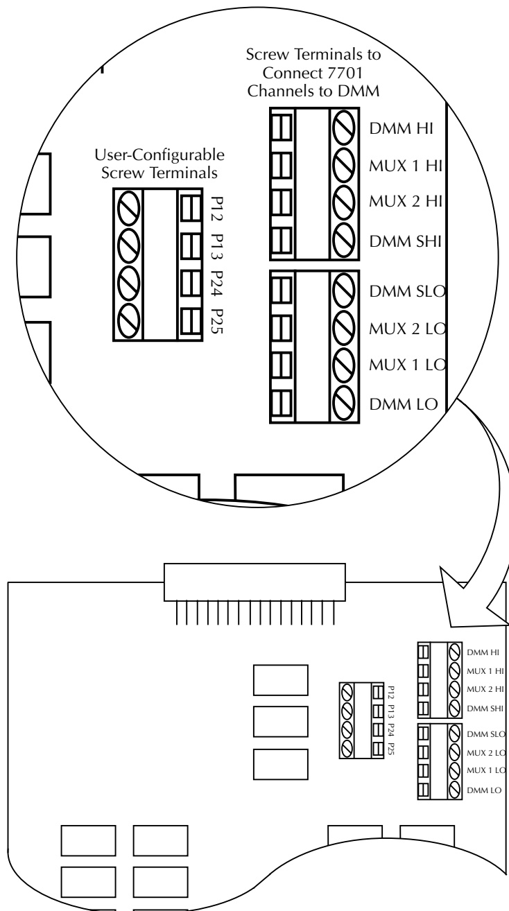
Figure 2 Model 7701 screw terminals
