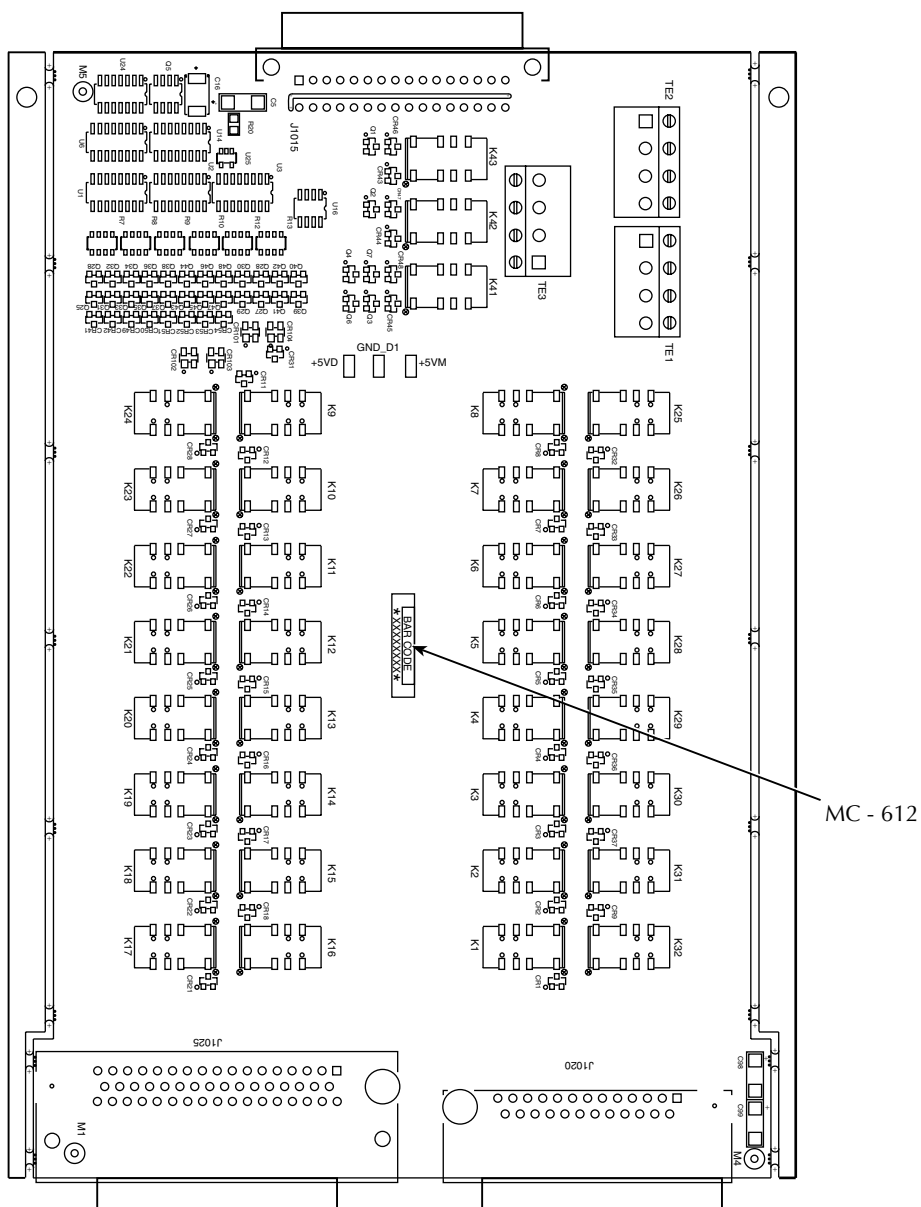
Figure 16 Model 7701 component layout (Side-06)
