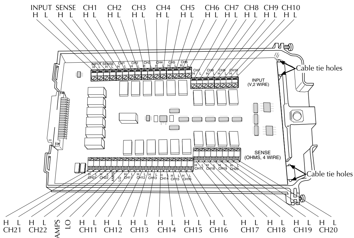
Model 7700 screw terminal channel designations
