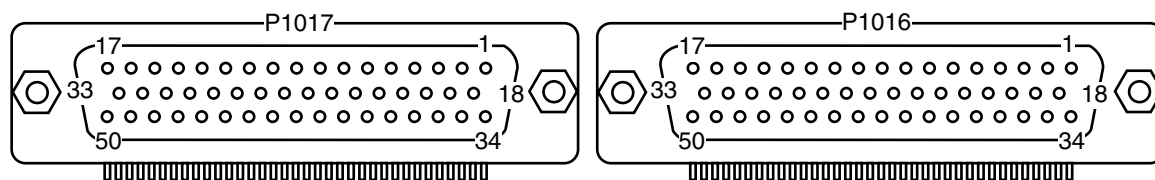
Rear view—Model 7703 Pinouts (P1016 and P1017)
