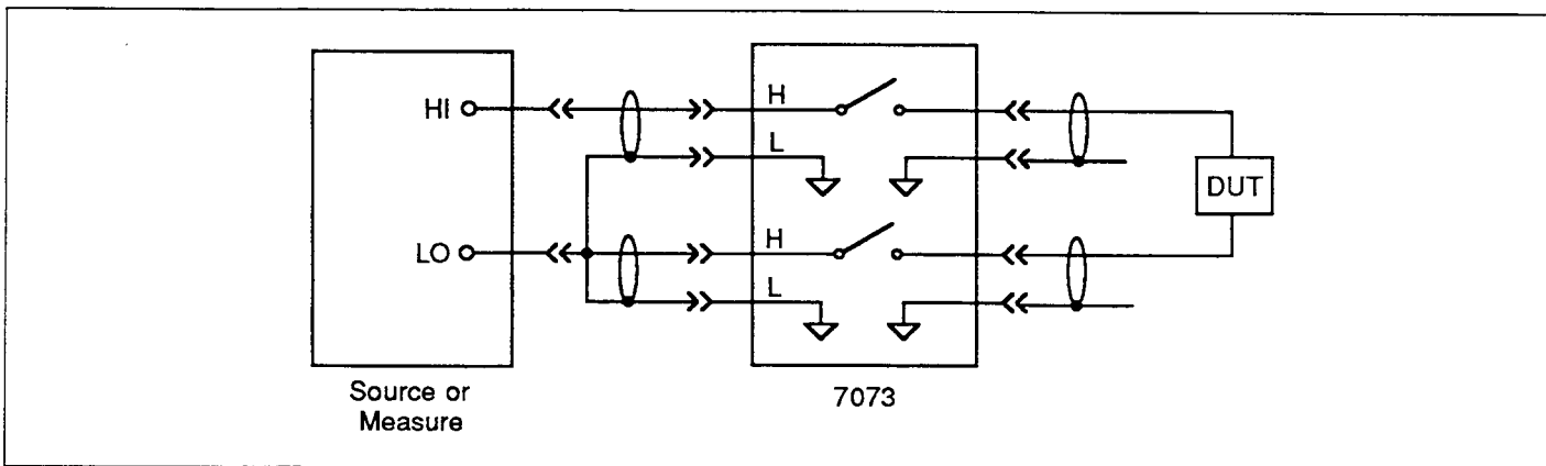
Figure 2-4. Differential (Shielded)
