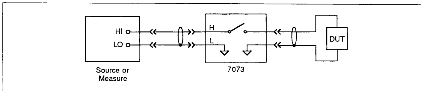
Figure 2-3. Single Ended
