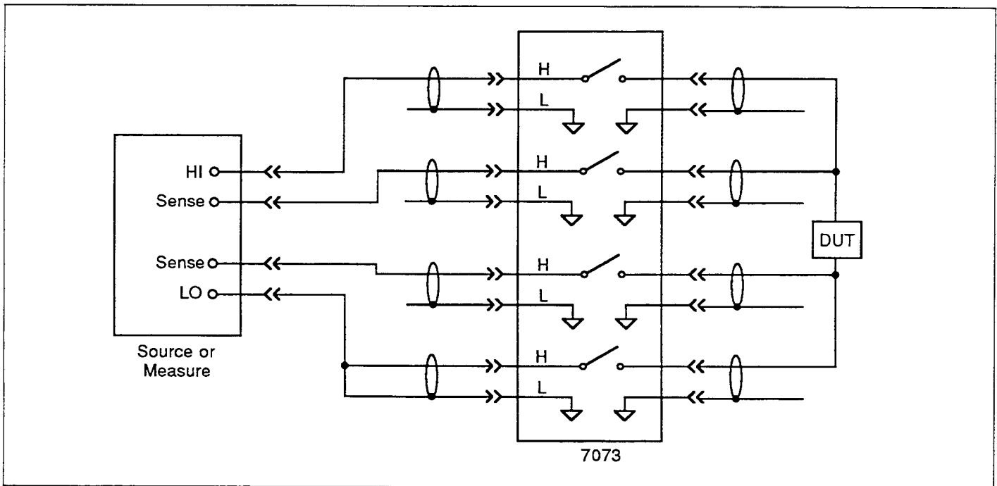
Figure 2-5. Sensing
