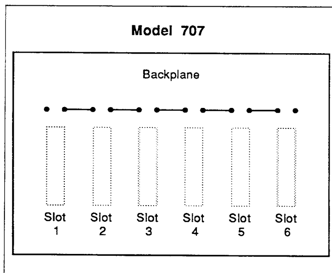
Figure 2-7. Model 707 Backplane Configuration for Model 7073 Cards
