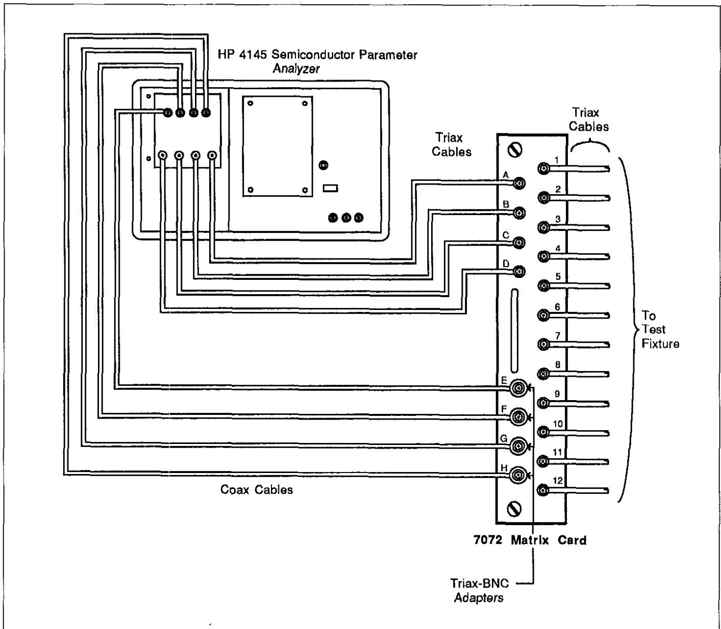
Figure 3-11. SPA Connections
