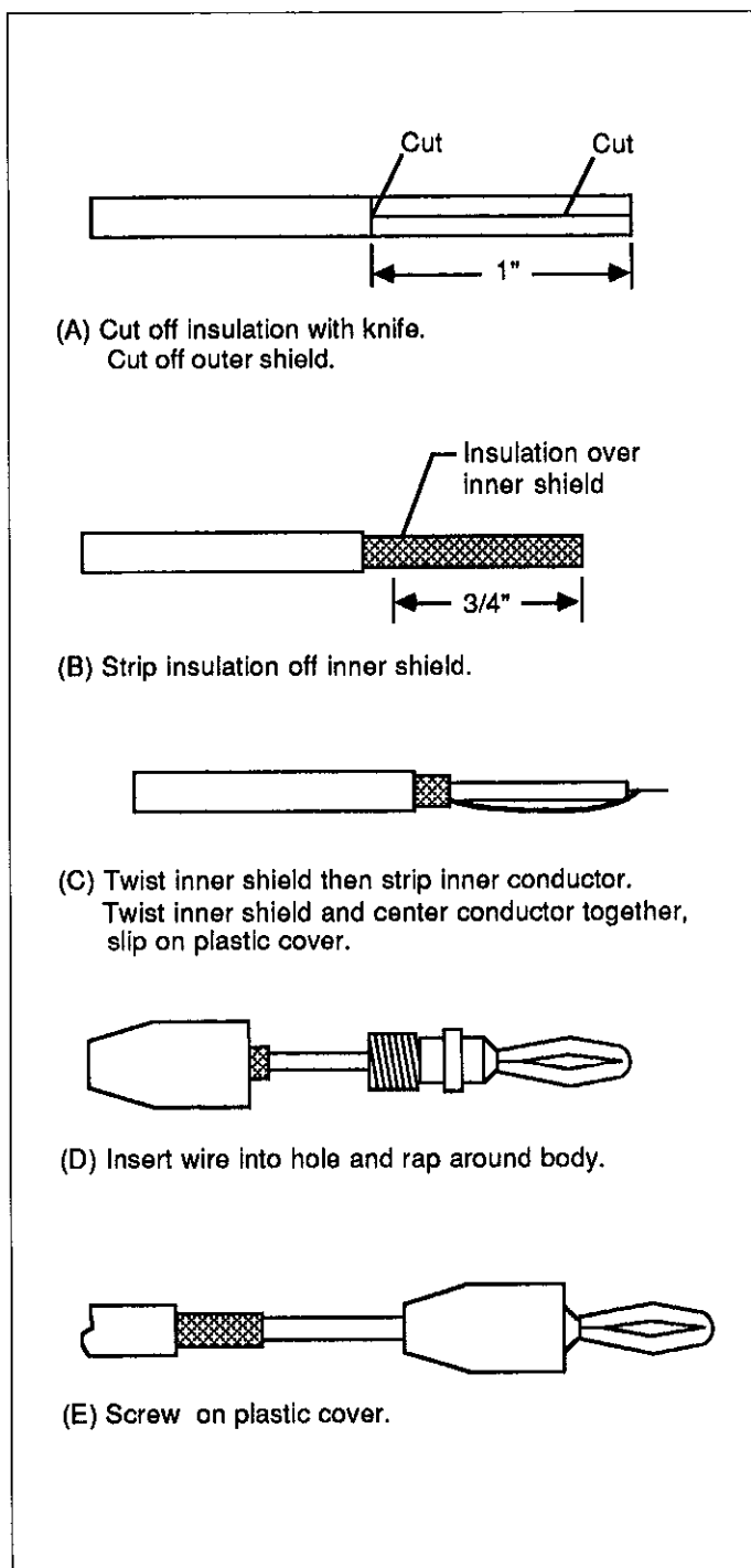
Figure 4-5. Triaxial Cable Preparation
