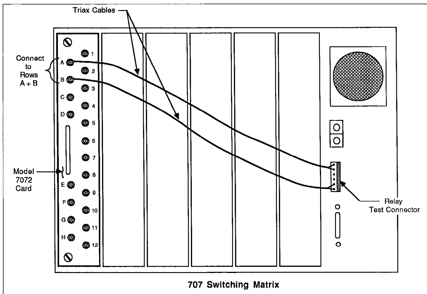
Figure 4-2. Connecting the Test Cable to the Model 7072
