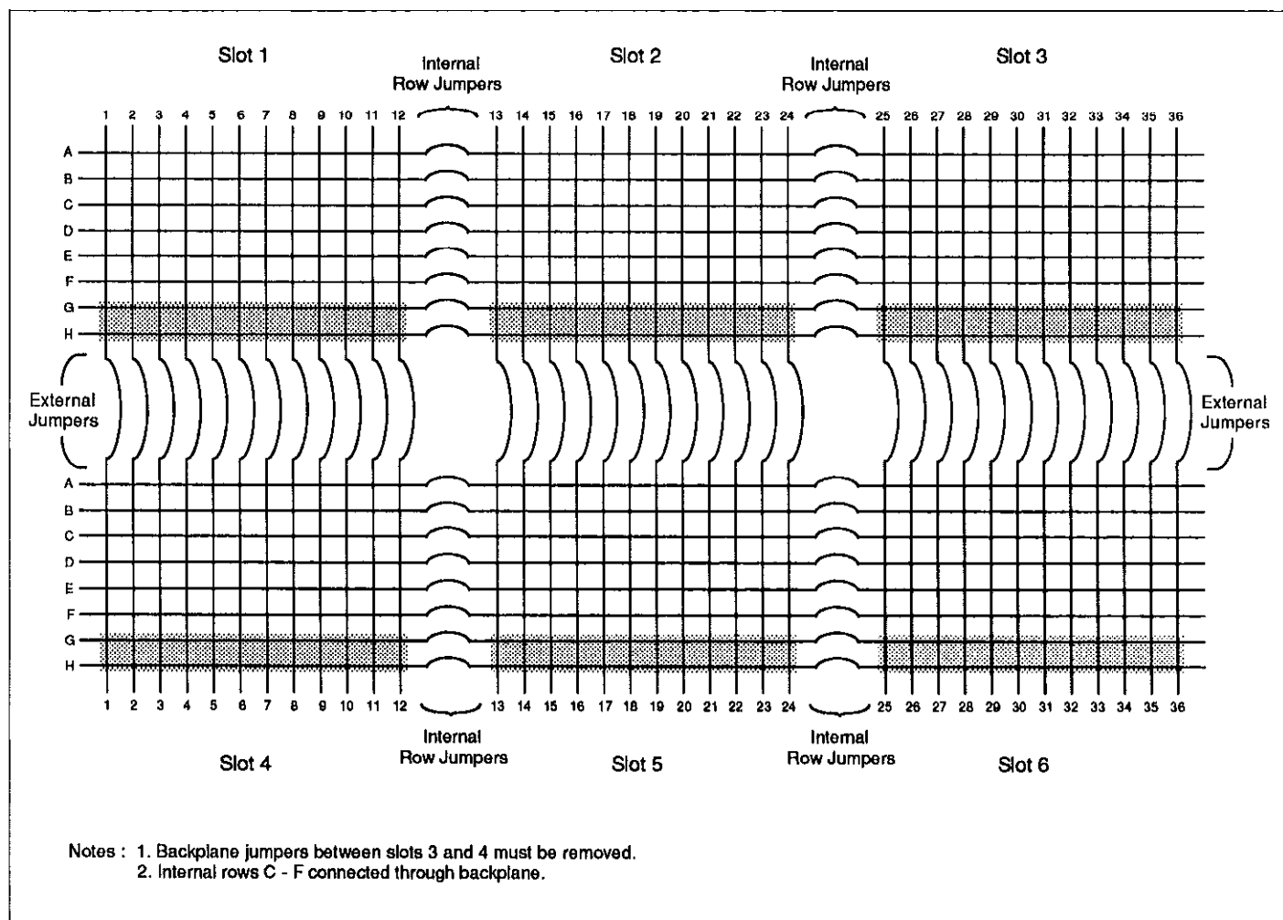
Figure 2-17. 16 \times 36 Matrix Constructed by External Jumpering
