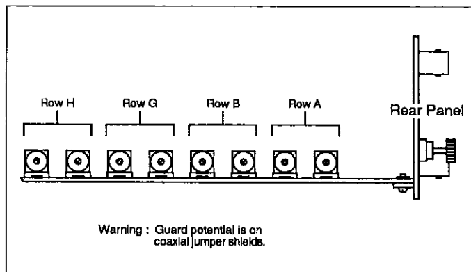
Figure 2-15. Jumper Connector Locations
