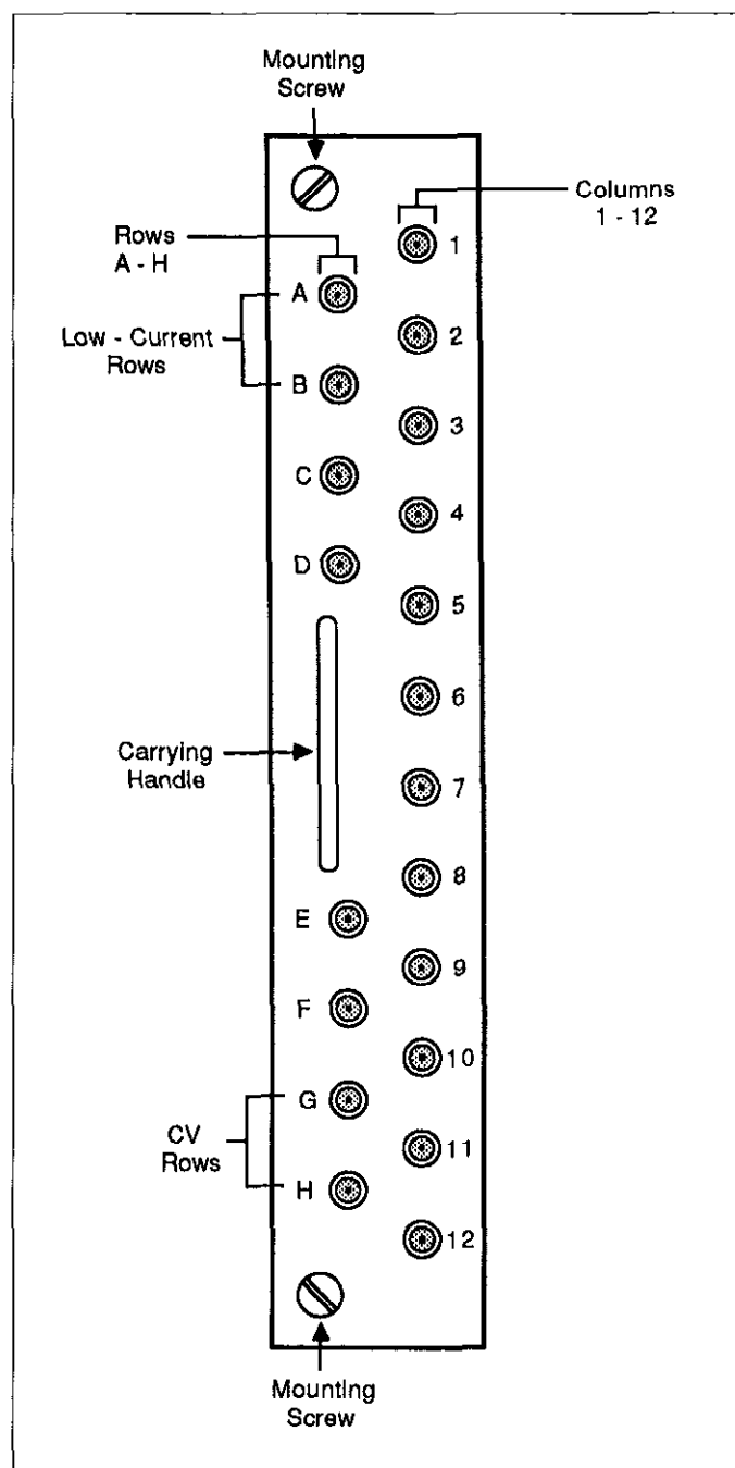
Figure 2-2. Card Connectors
