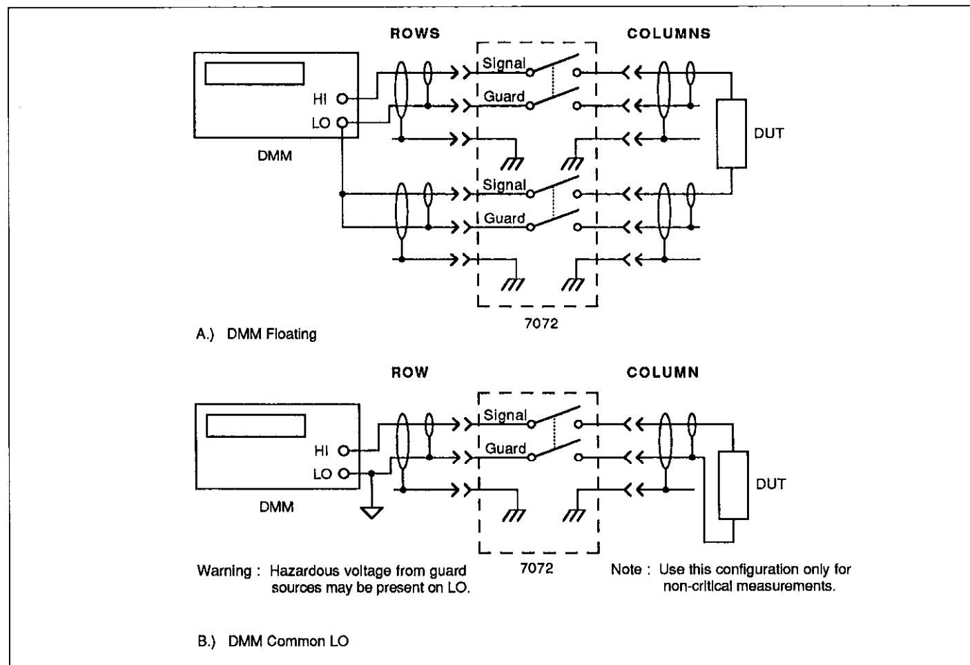
Figure 2-5. General Instrument Connections (A-B)
