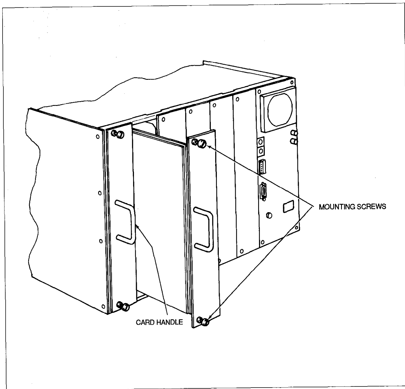
Figure 2-1. Model 7072 Installation
