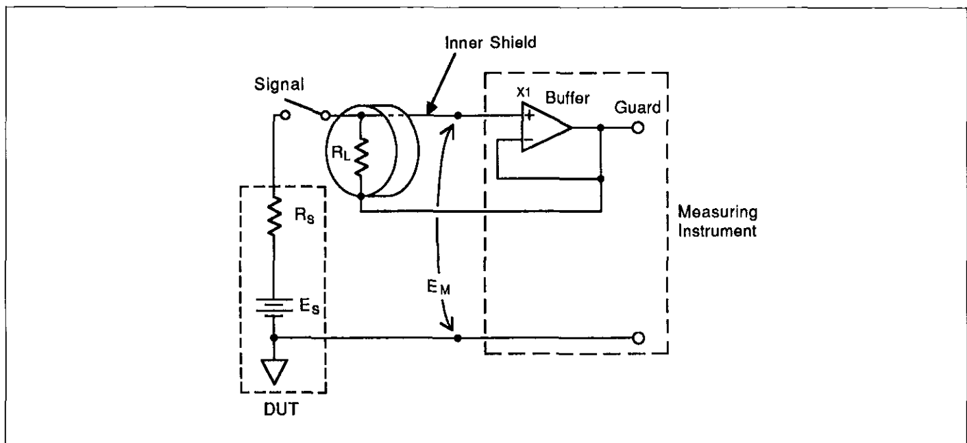
Figure 2-23. Guarded Circuit
