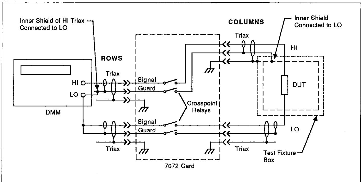
Figure 2-21. Shielding Example
