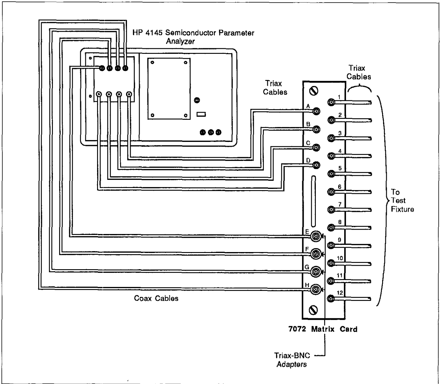
Figure 3-11. SPA Connections
