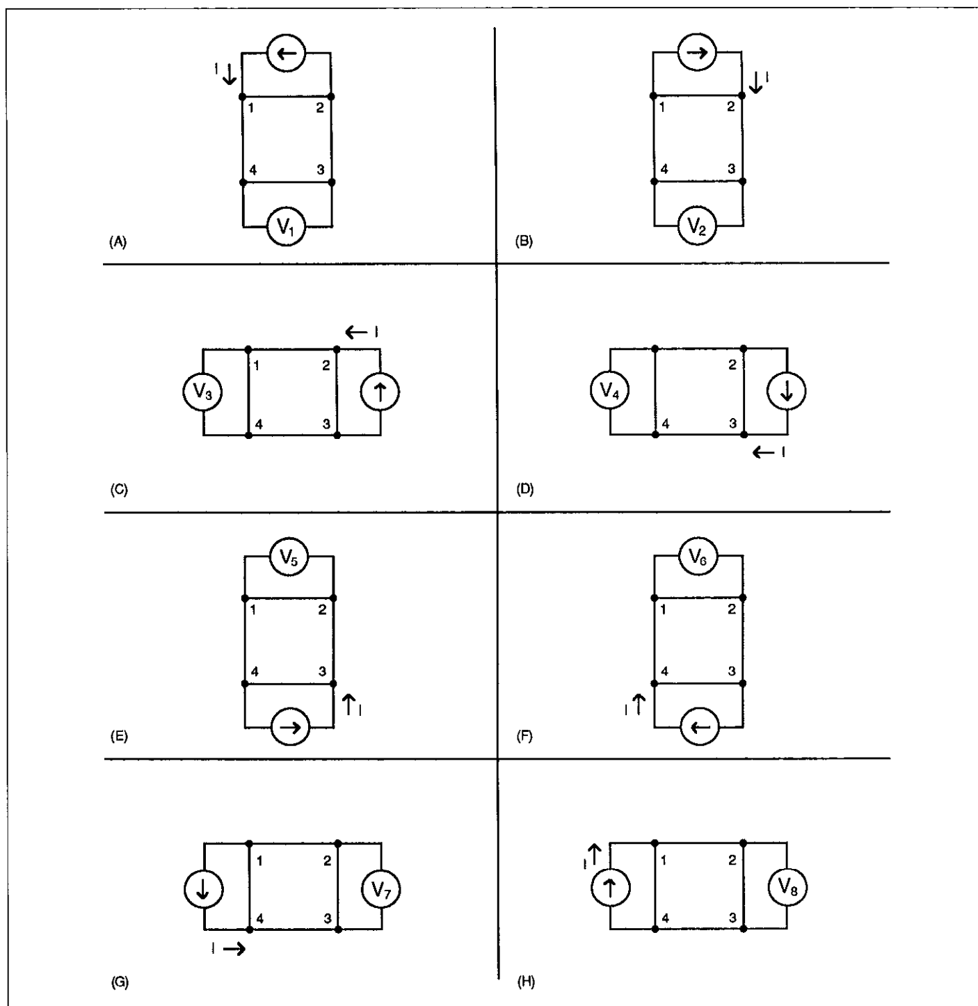
Figure 3-9. Resistivity Measurement Conventions
