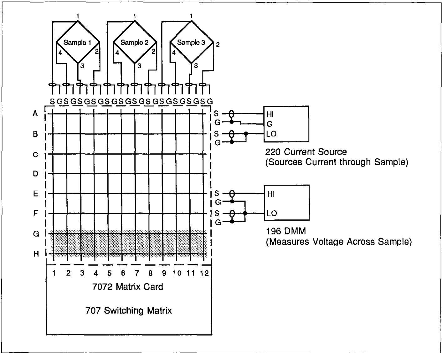
Figure 3-8. Resistivity Test Configuration
