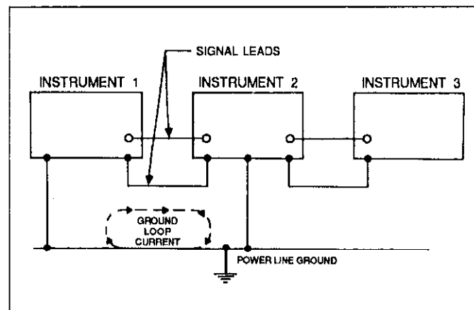
Figure 2-19. Power Line Ground Loops
