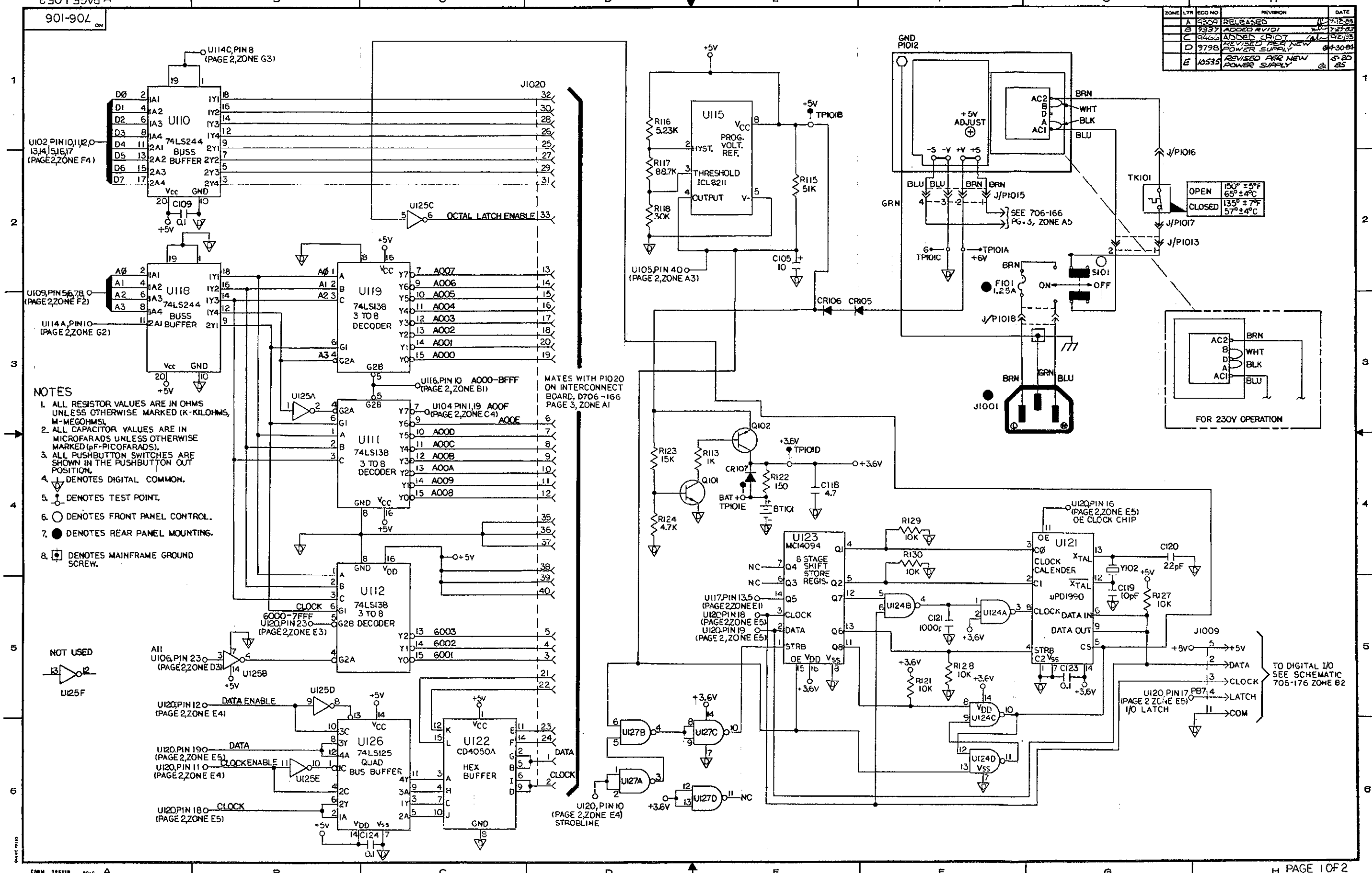
Figure 6-7. Mother Board, Schematic Diagram, Dwg. No. 706-106 (sheet 1 of 2)
