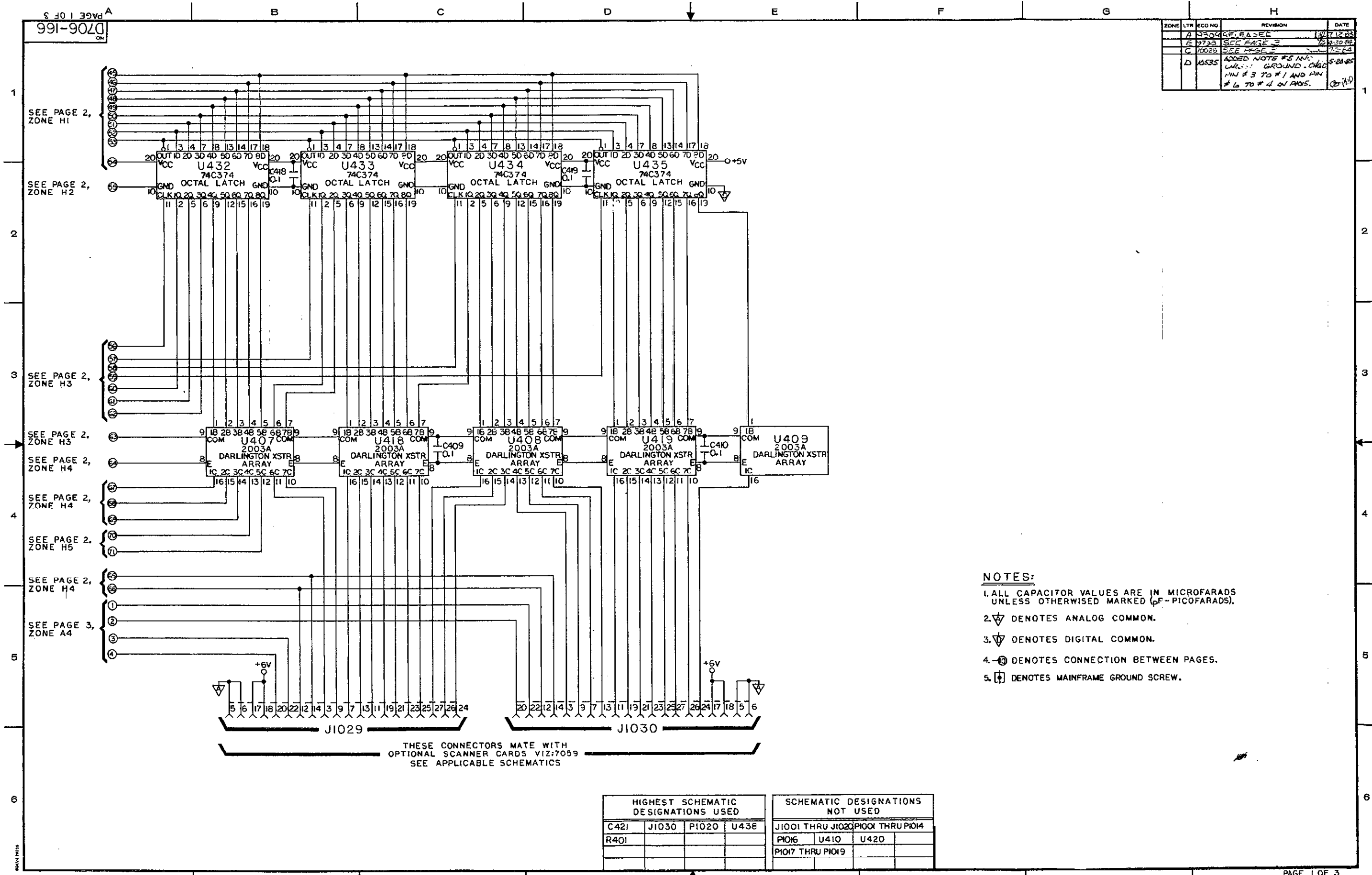
Figure 6-8. Interconnect Board, Schematic Diagram, Dwg. No. 706-166 (sheet 1 of 3)
