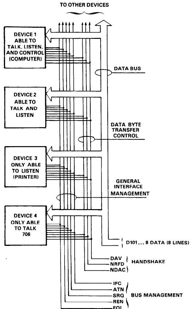
Figure 3-1. Bus Structure
