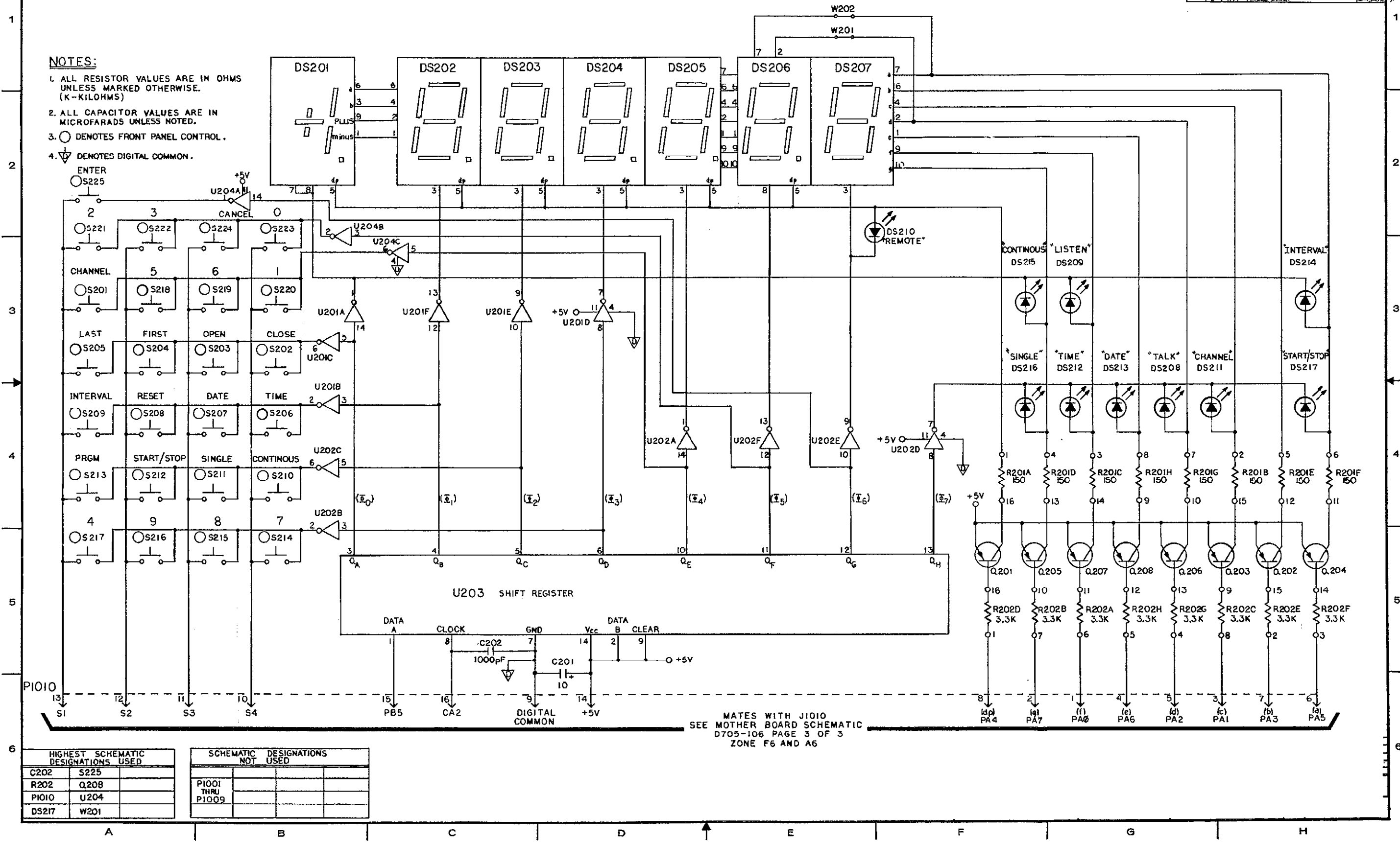
Figure 6-5. Display Board, Schematic Diagram Dwg. No. 705-116
