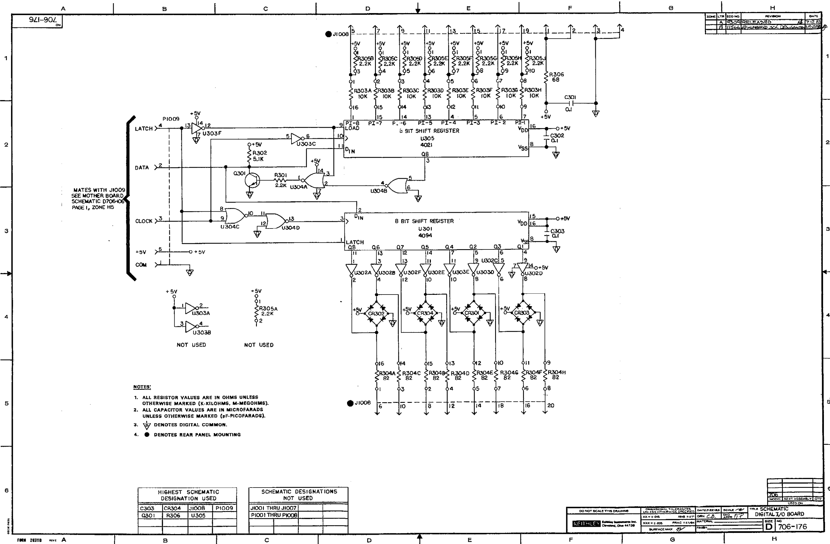
Figure 6-6. Digital I/O Board, Schematic Diagram, Dwg. No. 706-176
