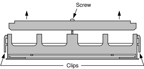
Figure 3-4 Cable clamp for screw terminal connector card
