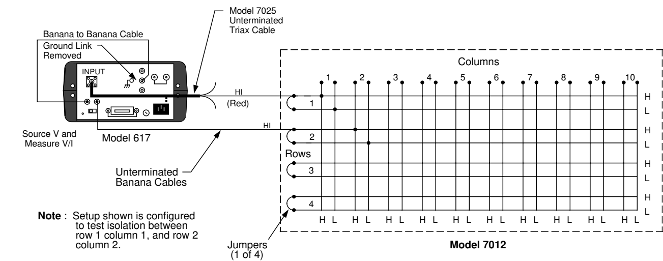
Figure 5-5 Path isolation testing (guarded)
