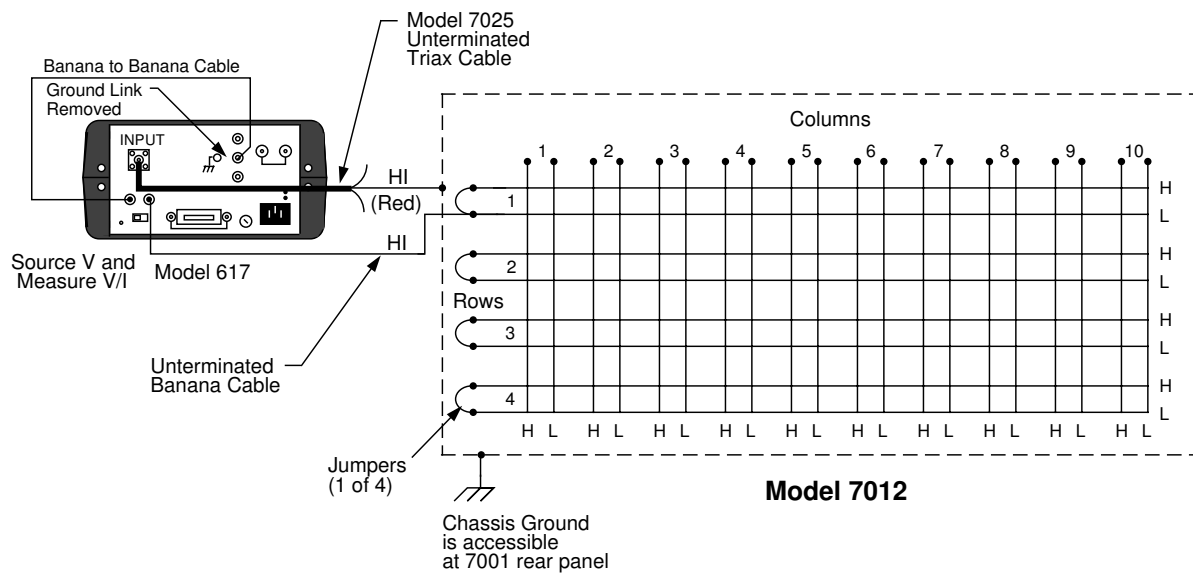
Figure 5-7 Common-mode isolation testing
