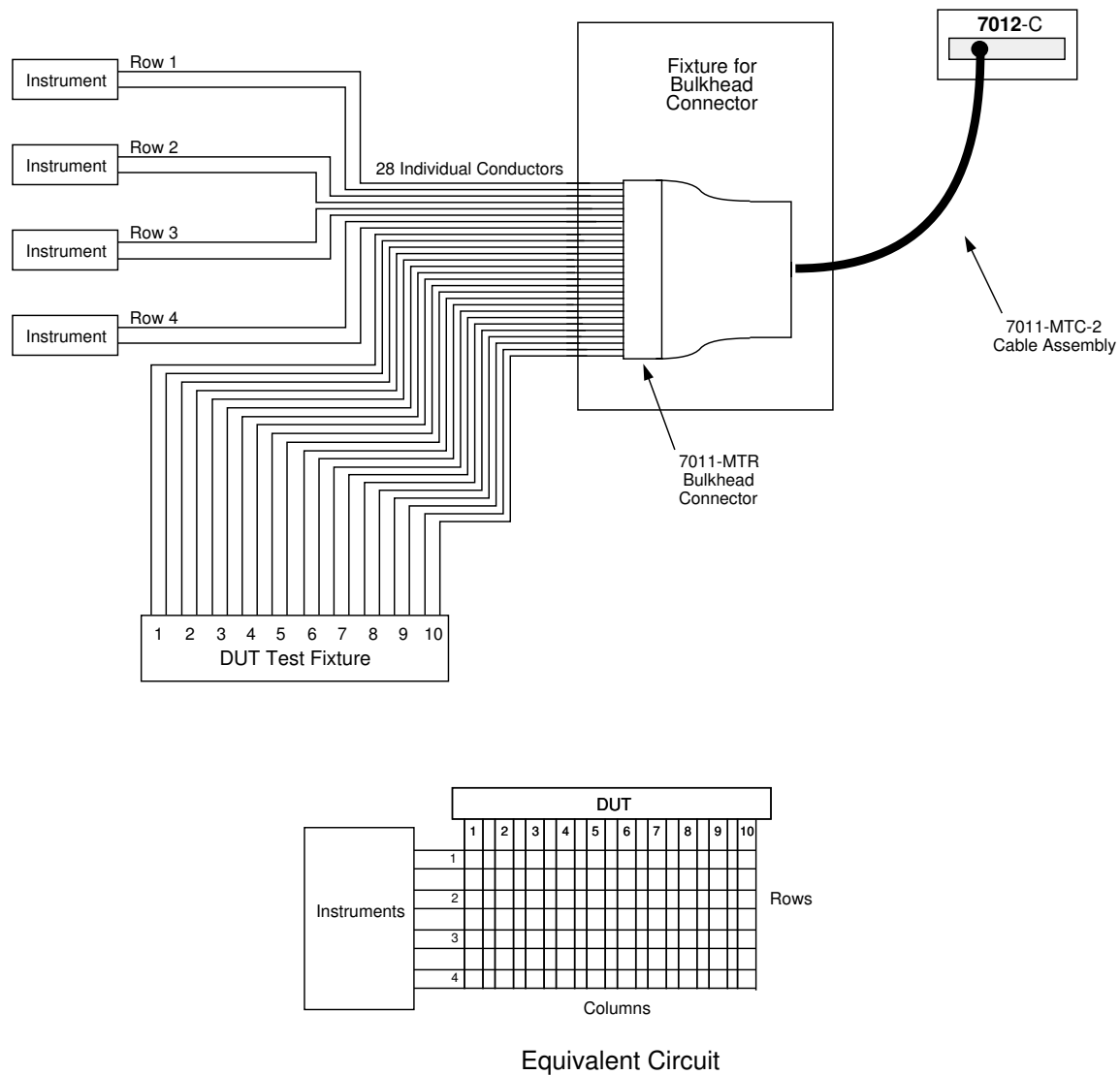
Figure 3-9 Single card system example (multi-pin connector card)
