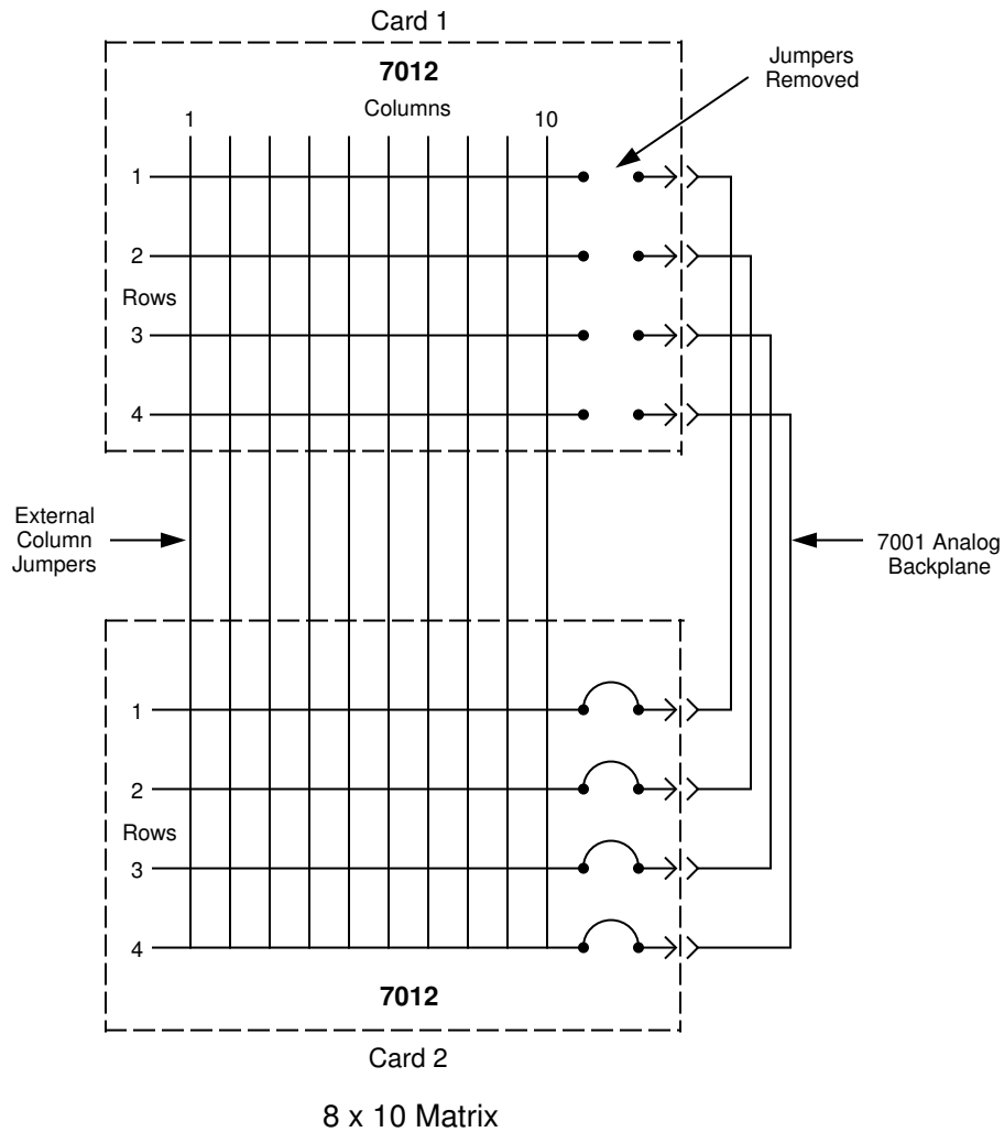
Figure 2-10 Wide matrix example (8 × 10)
