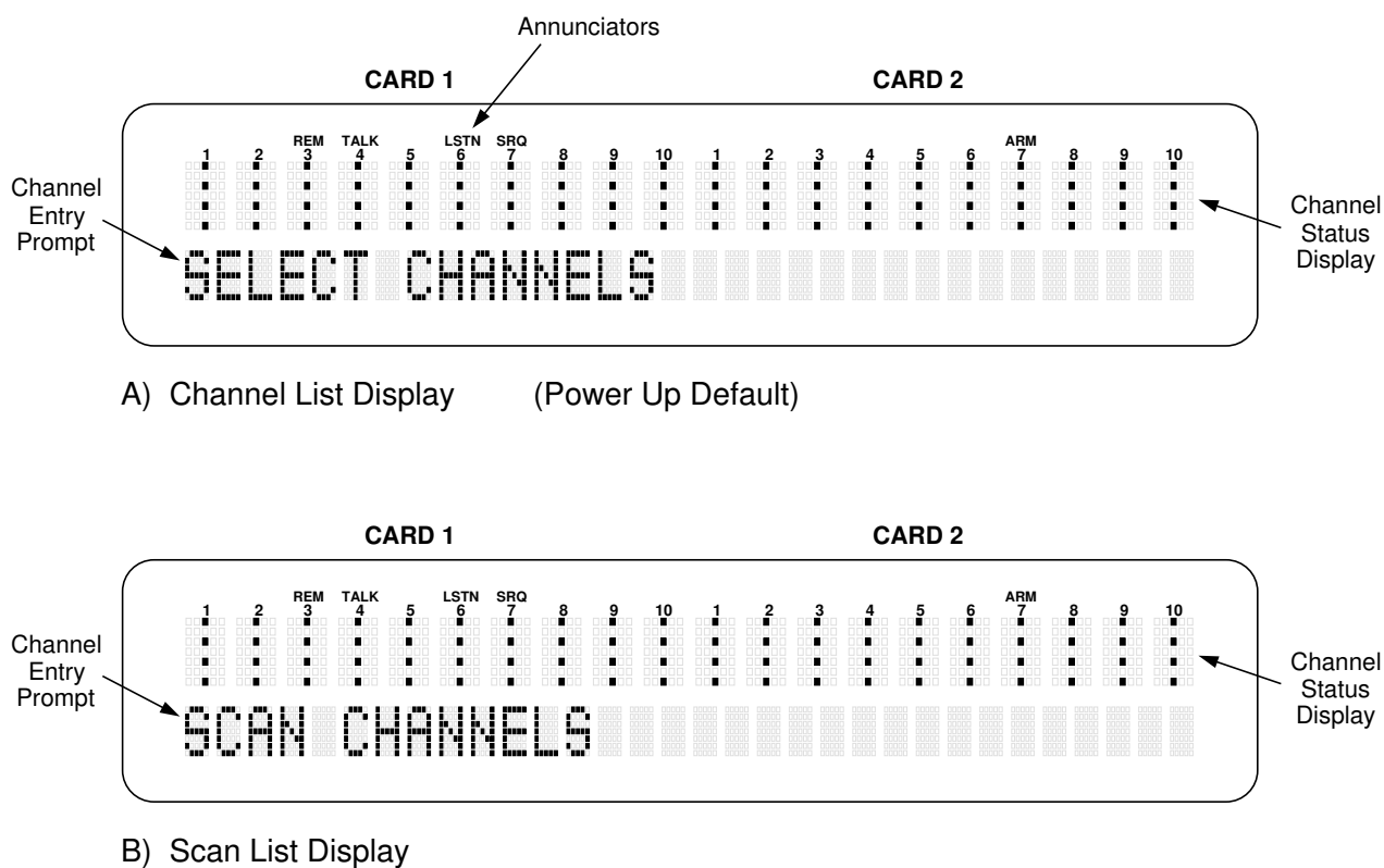
Figure 4-1 Display format
