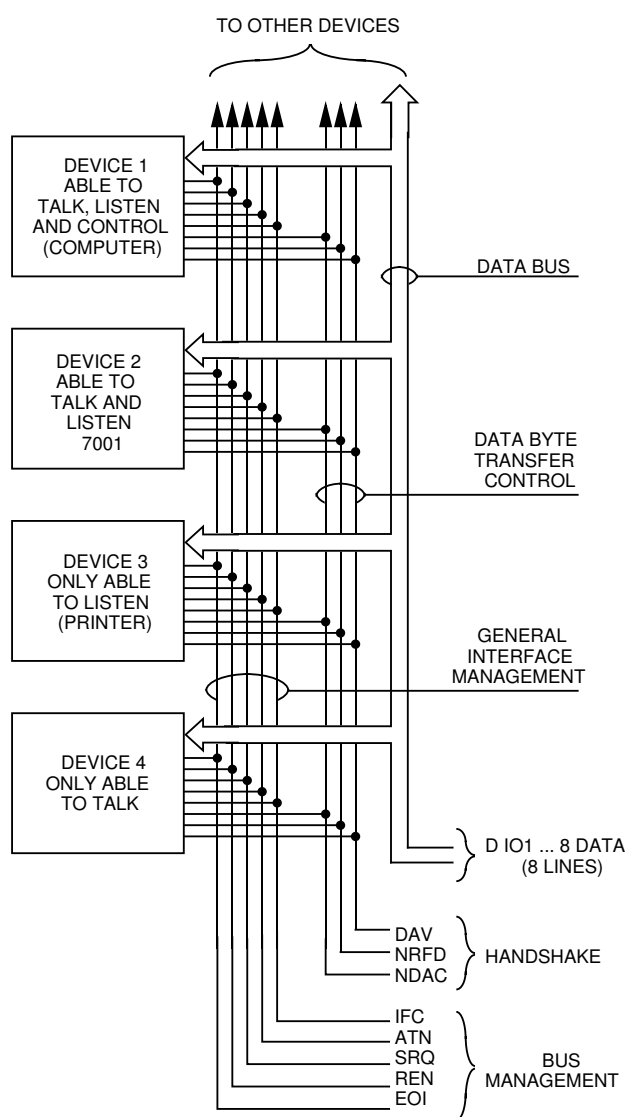
Figure D-1 IEEE-488 bus configuration
