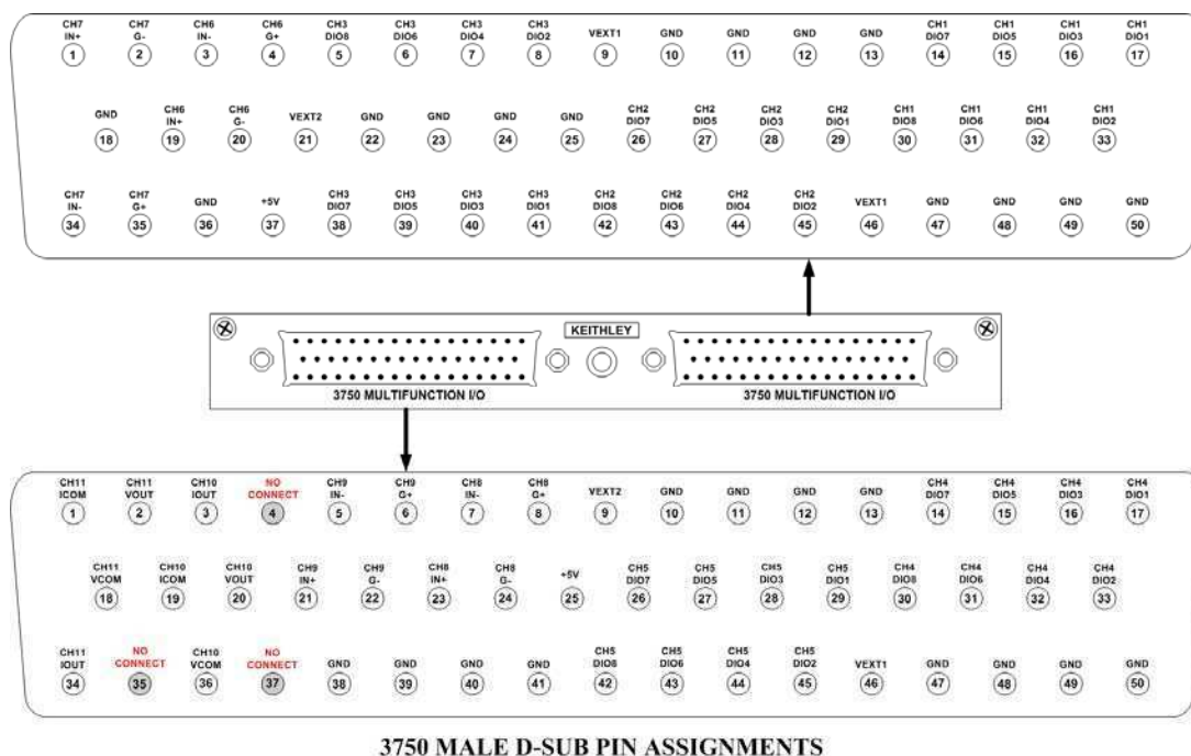
Figure 2: Model 3750 connection information
