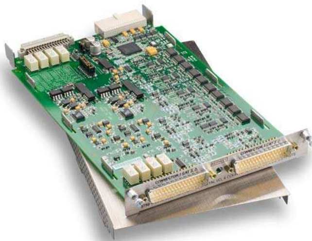
Figure 1: Model 3750 Multifunction I/O Card
