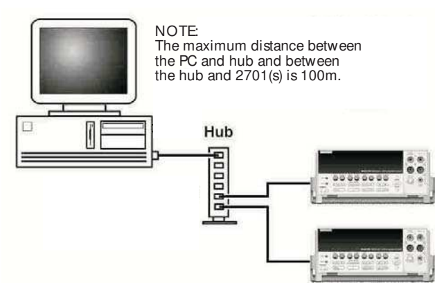
Figure 2-2 Hub to Model 2701
