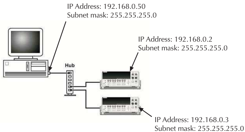
Figure 3-1 IP address byte location sample
