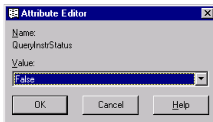
Figure 4-12 Attribute setting
