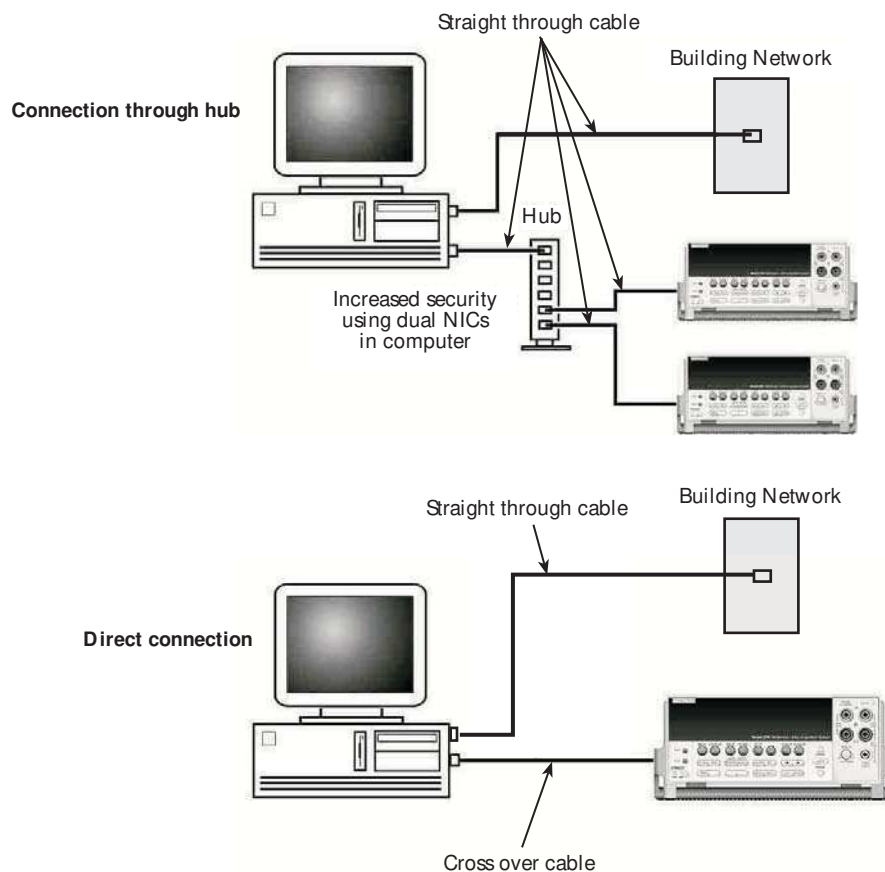
Figure 2-3 Dual NIC to Model 2701
