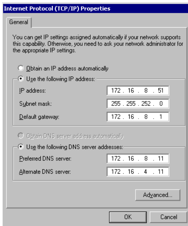
Figure 3-6 Windows 2000 Ethernet card settings
