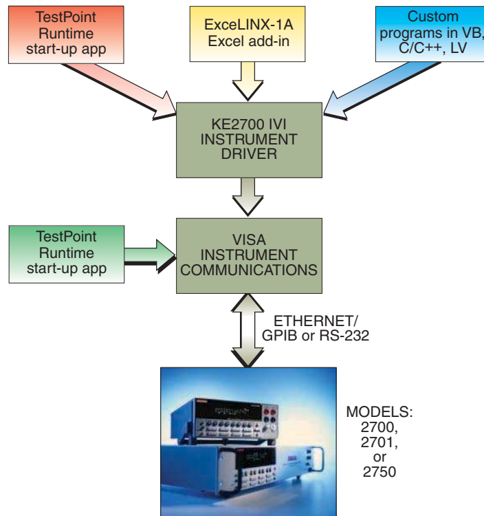
Figure 4-1 Software overview
