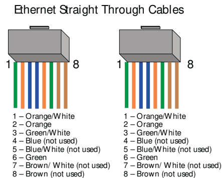
Straight through cables
