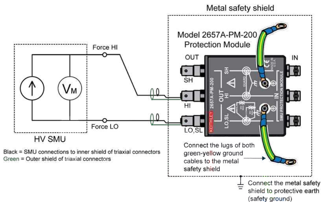
Figure 14: Connections for verification procedure F
