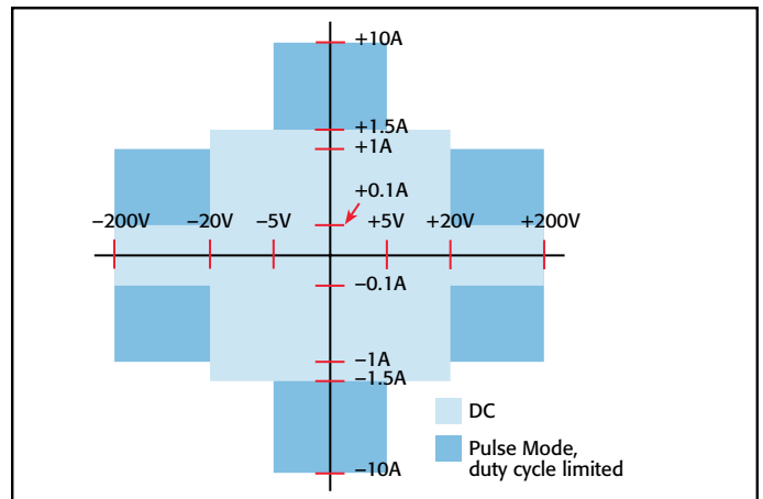
Models 2611 and 2612 I-V capability
