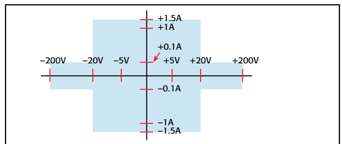
Models 2635 and 2636 I-V capability
