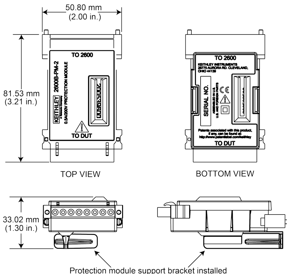
Figure 2: Model 2600B-PM-2 dimensions
