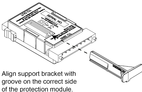
Figure 4: Installing the support bracket for use in channel B
