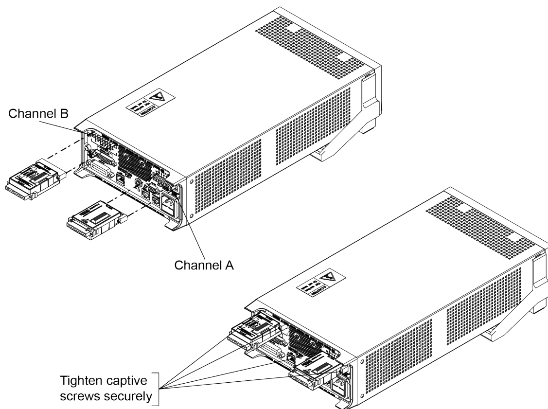
Figure 5: Connecting the Model 2600B-PM-2 to your SMU
