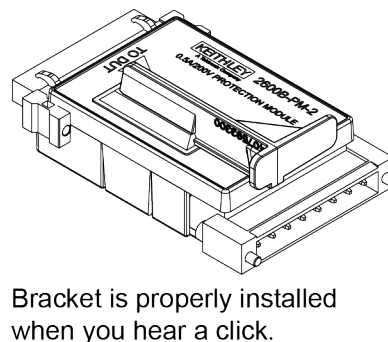
Figure 4: Installing the support bracket for use in channel B
