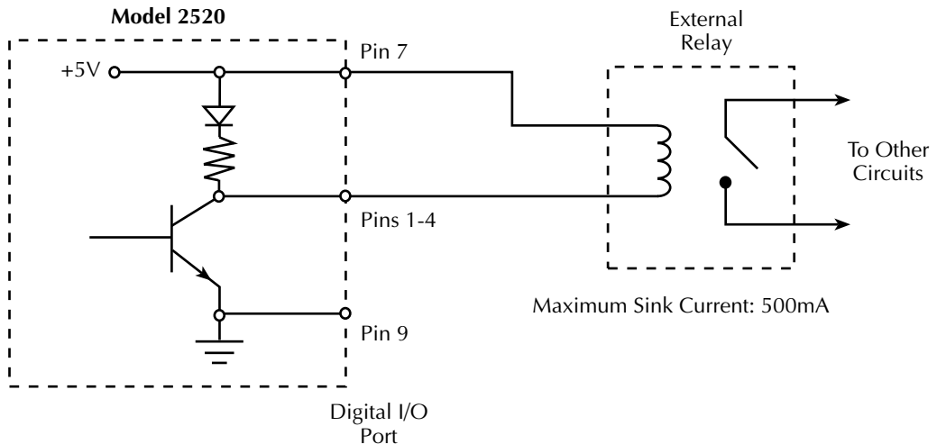
Figure 9-2 Sink operation
