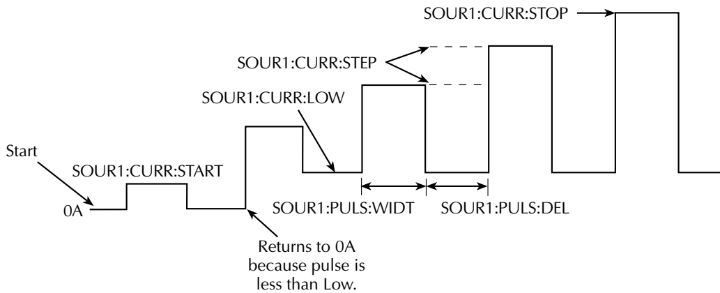
Figure 5-6 Remote staircase sweep mode pulse parameters
