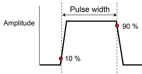
Figure 84: Pulse width
