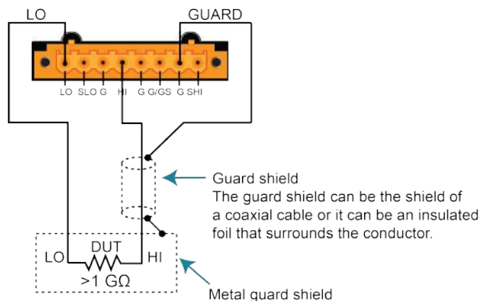
Figure 115: 2461 high-impedance guarding
