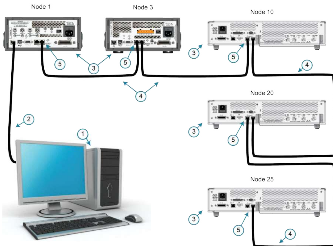
Figure 152: TSP-Link connections
