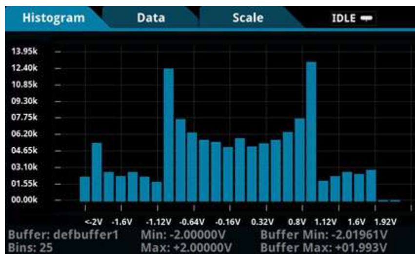
Figure 48: 2461 Histogram
