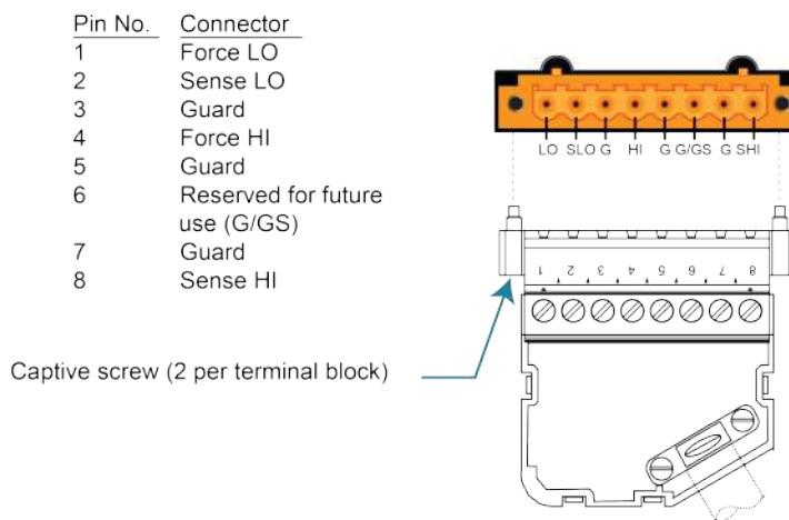
Figure 55: 2461 rear-panel screw terminal connections
