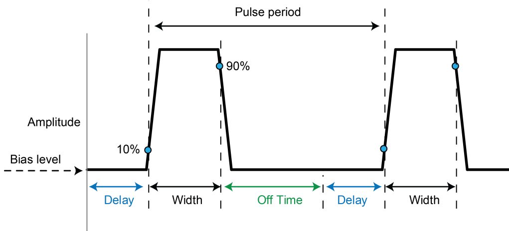
Figure 86: Pulse period
