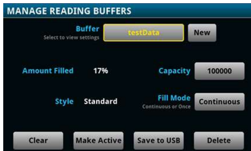
Figure 183: MANAGE READING BUFFERS window
