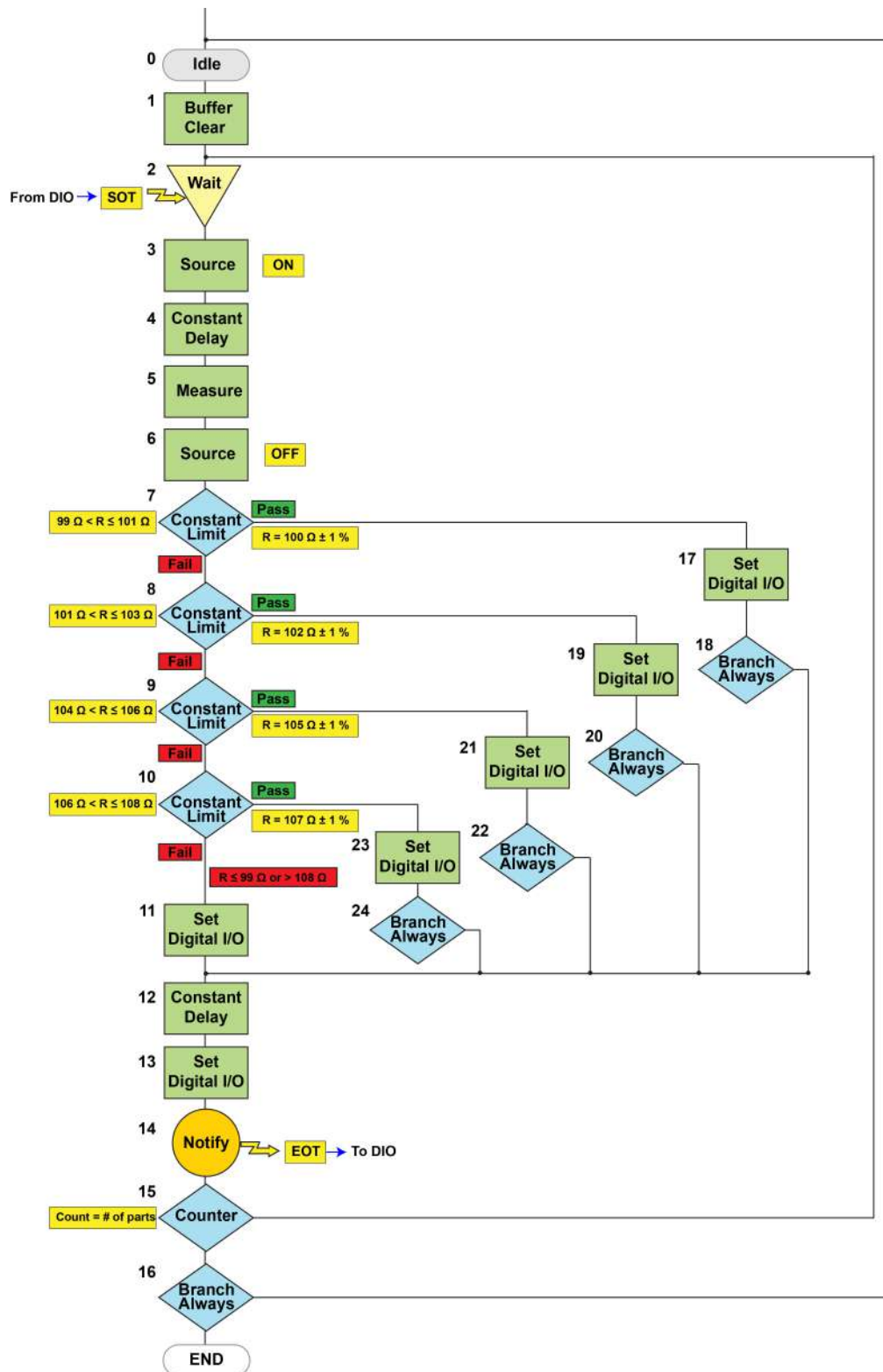
Figure 100: Resistor sorting example trigger model
