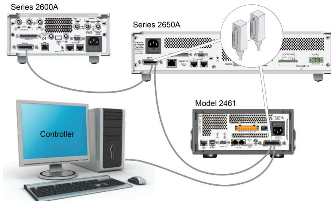
Figure 11: Model 2461 IEEE-488 connections
