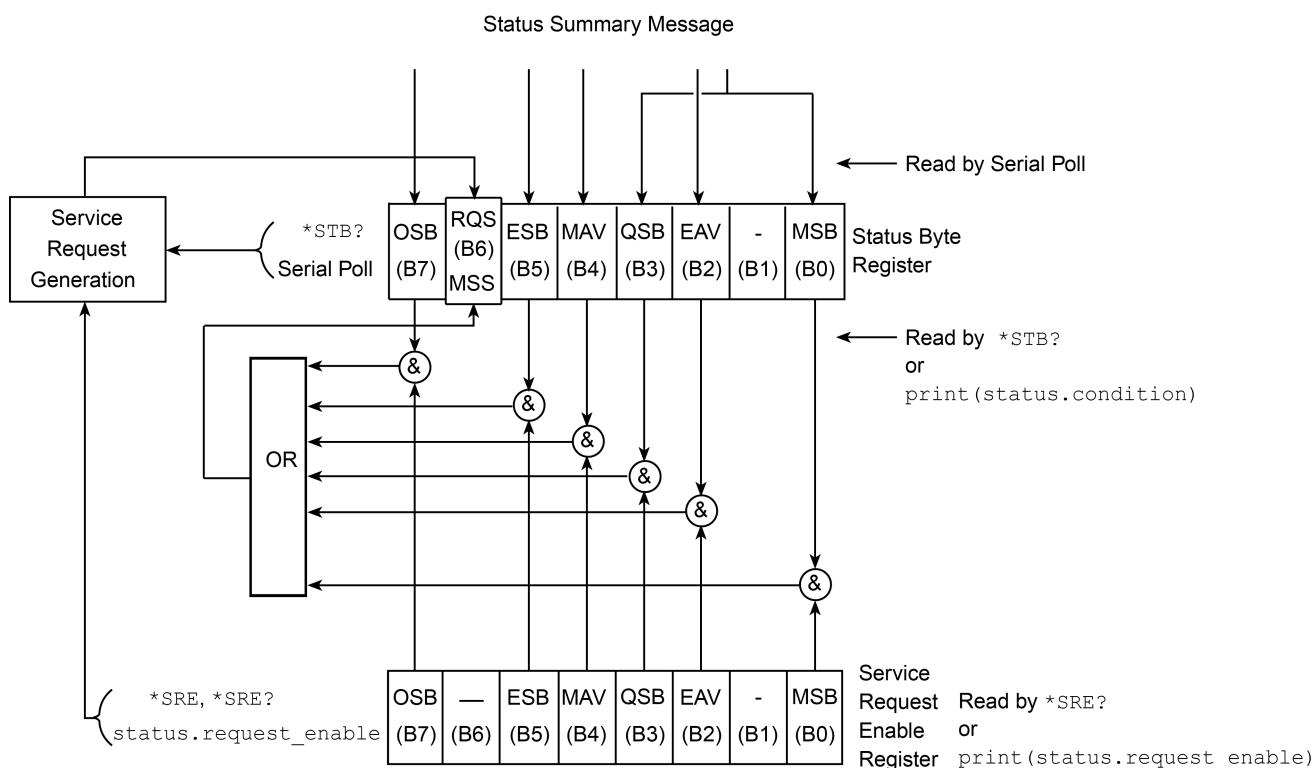
Figure 180: 2461 Status Byte Register
