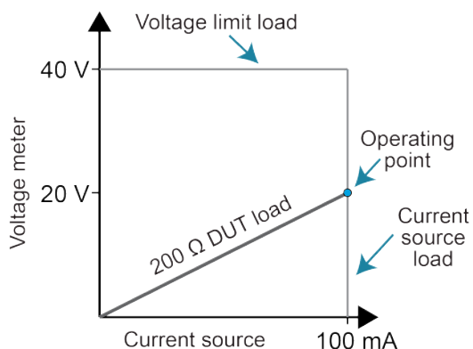
Figure 107: 2461 limit boundary example — normal
