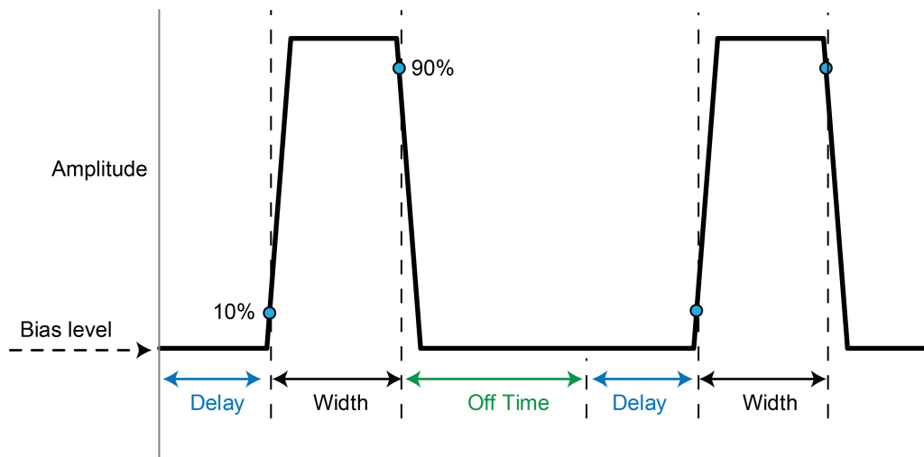
Figure 85: Pulse delay and off time
