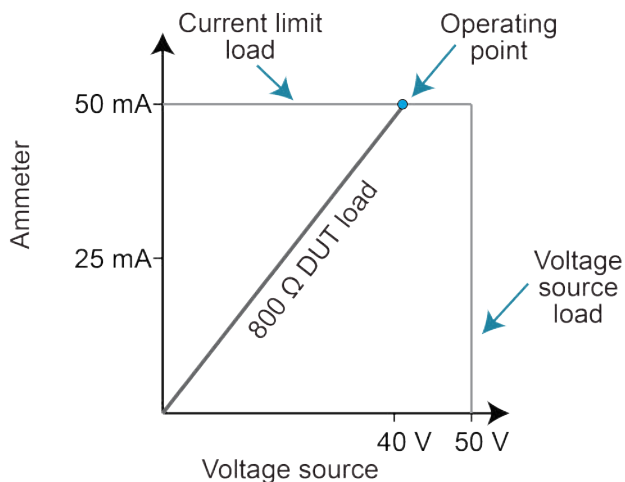
Figure 110: 2461 current limit boundary example limited
