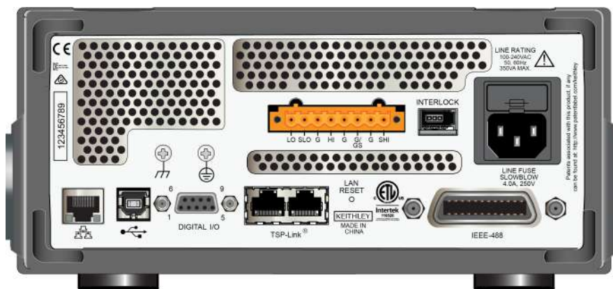
Figure 9: 2461 rear panel
