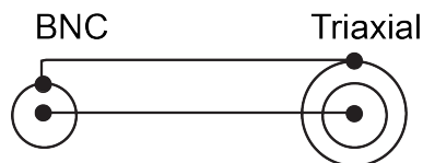
Figure 2: Model 237-BNC-TRX Schematic
