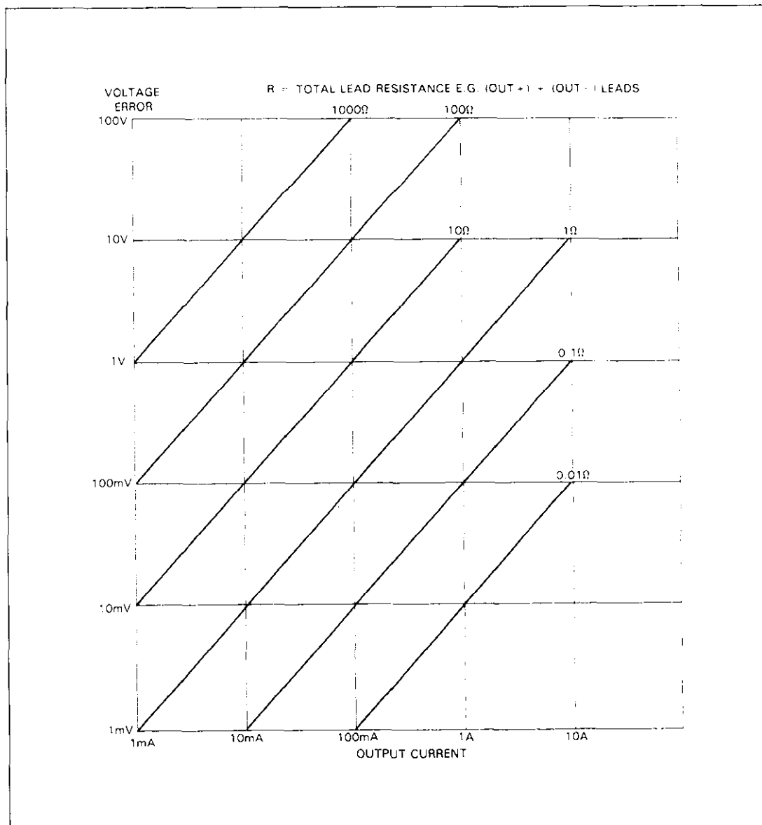
Figure 4. Voltage Error Using Local Sensing
