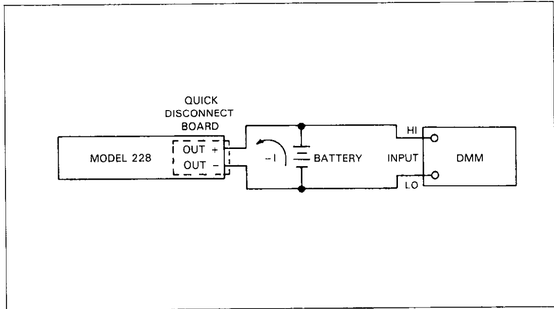
Figure 11. Data Logging Configuration
