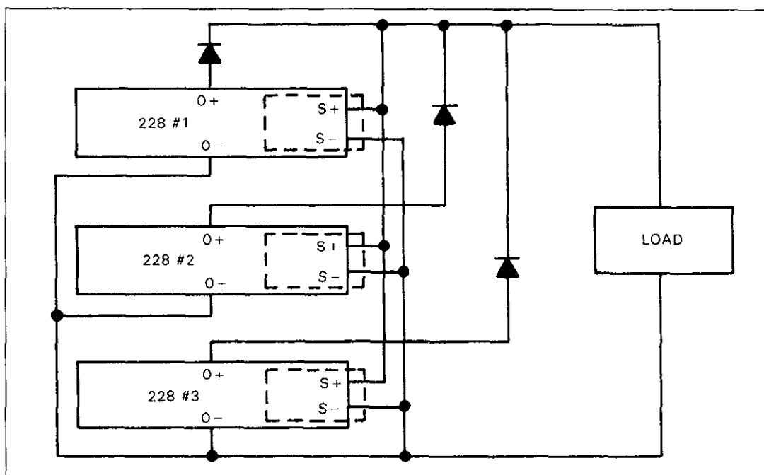
Figure 16. Configuring Three or More Model 228s for Higher Current
