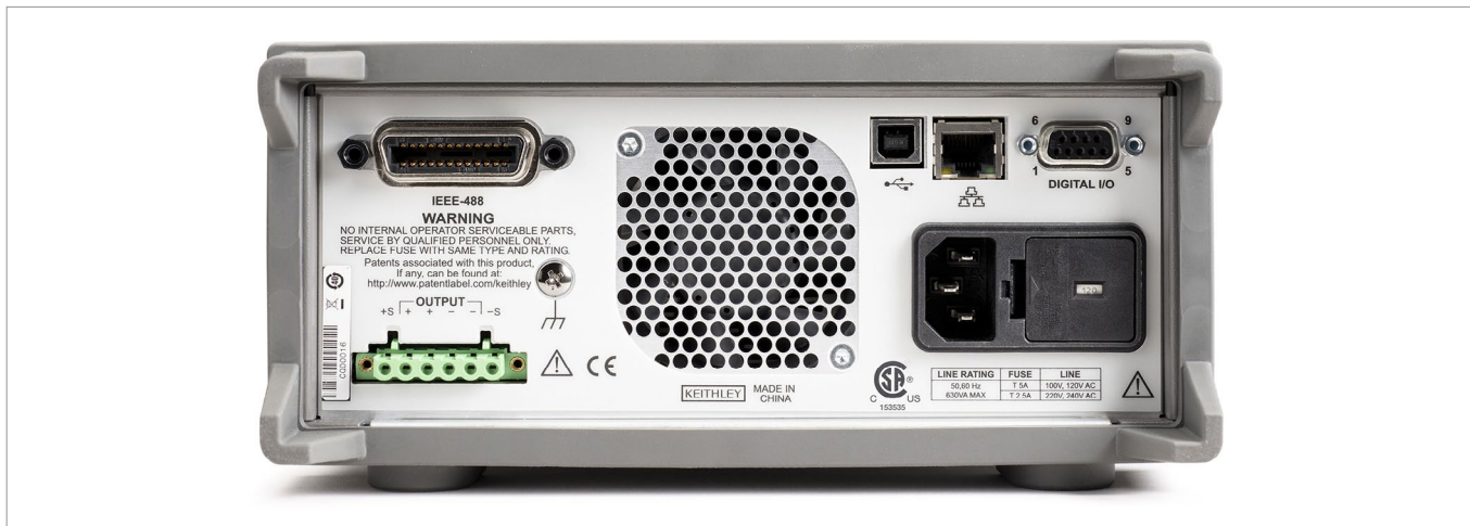
Figure 11. Series 2280S rear panel showing the rear output connector with remote sense inputs, digital I/O, and the three interfaces (GPIB, USB, and LAN).
