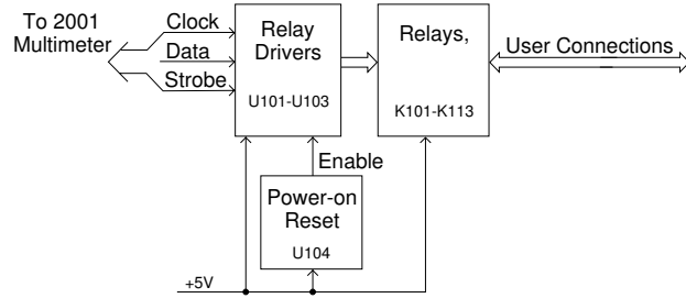
Figure 4-9 Block diagram
