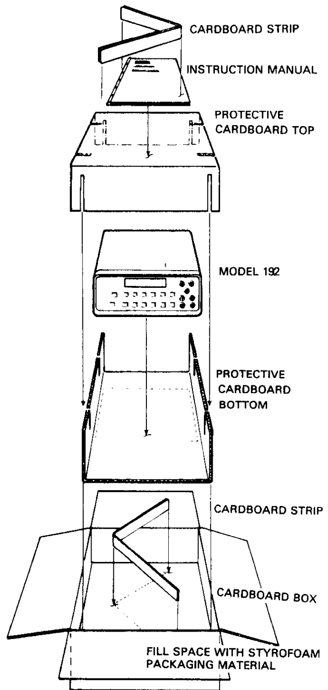
Figure 1-1. Instrument Packaging
