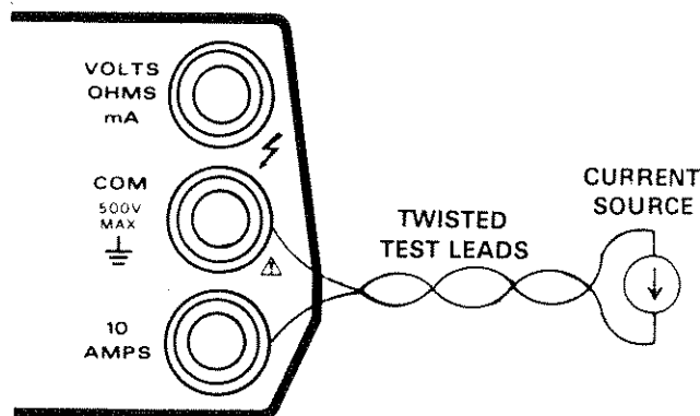
Figure 2-5. Current Measurements Between 2000mA and 20A
