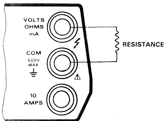
Figure 2-4. Resistance Measurements
