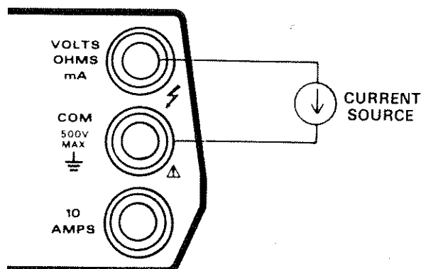
Figure 2-6. Current Measurements up to 2000mA
