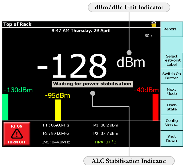
Figure 10: Power Stabilisation
