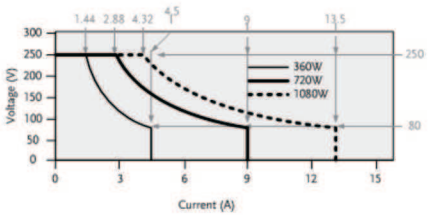
PSW 250V Series Operating Area
