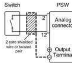
External Switch Control of the Main Power Shut-down
