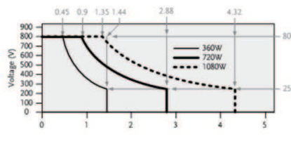
PSW 800V Series Operating Area
