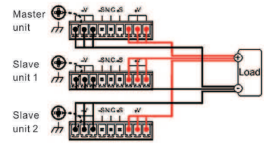
Parallel Connection
