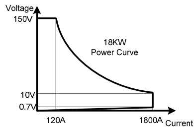
PEL-5018C-150-1800 power contour
