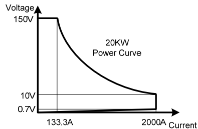
PEL-5020C-150-2000 power contour
