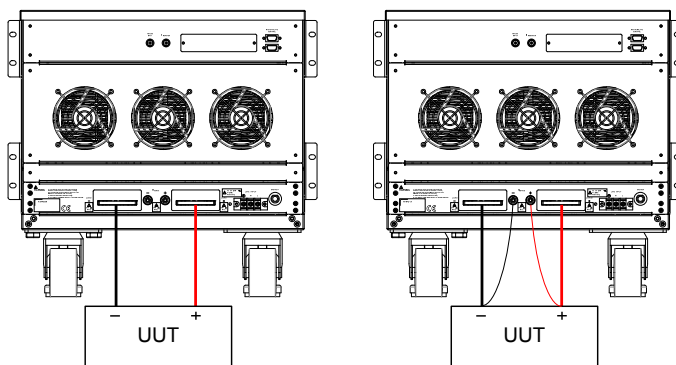
Typical connection of PEL-5000C series load module
