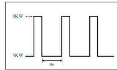
Example the Waveform of Load
