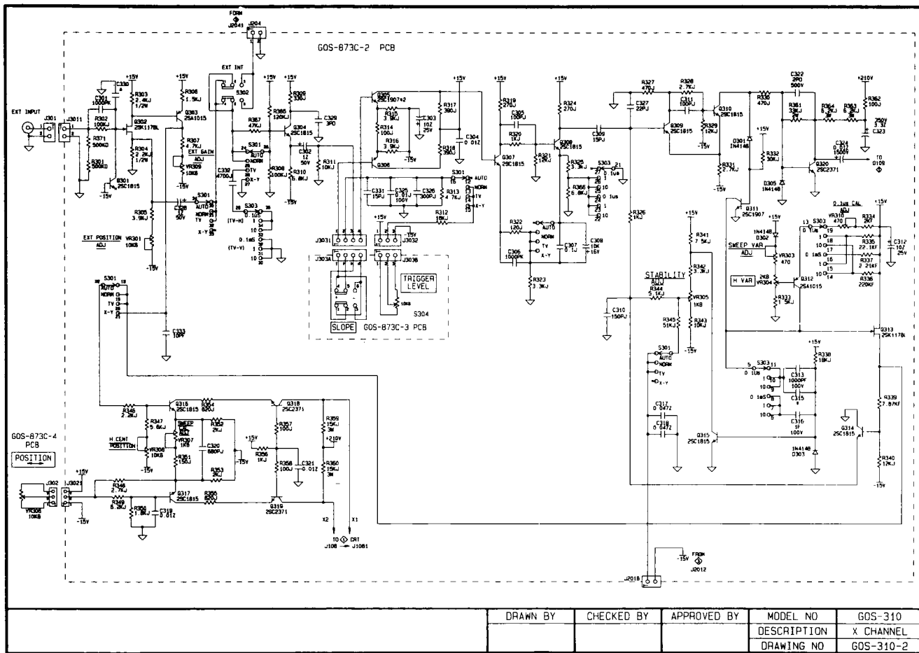
2.Horizontal Amplifier.
