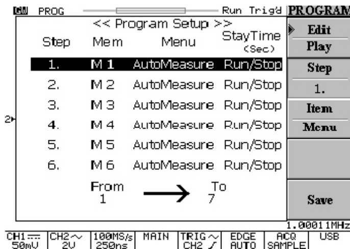
Figure 5-31: Enter to program mode
