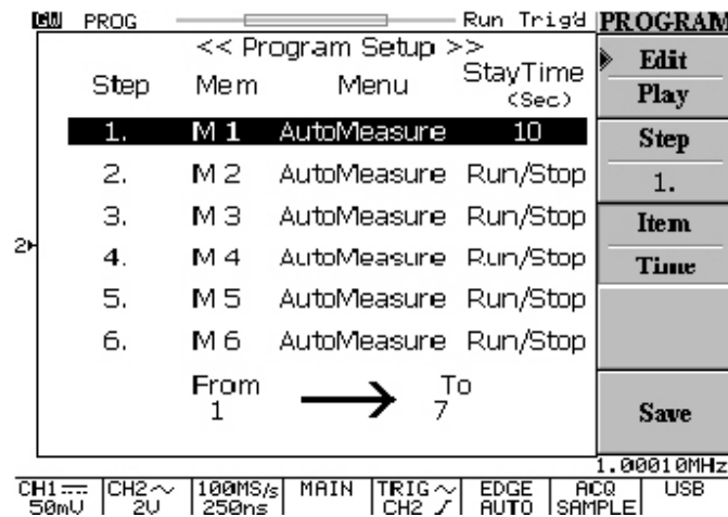
Figure 5-32: Editing the program condition of step one
