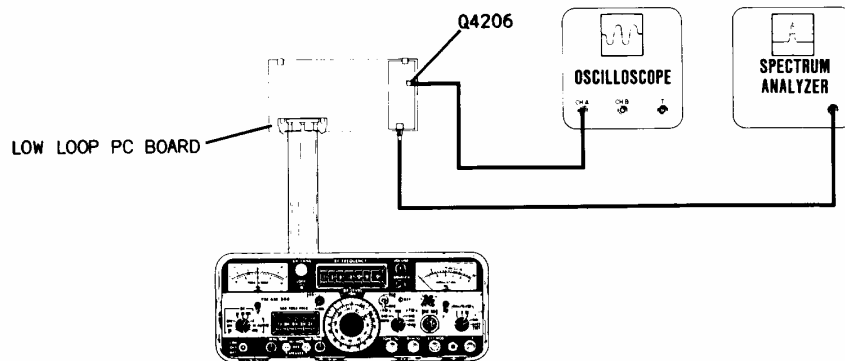
Figure 7-7 Low Loop Synthesizer Test Set-up
