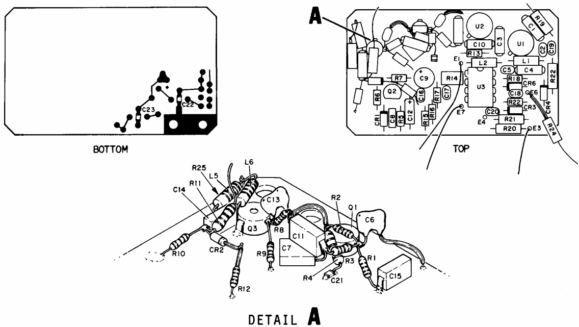
Figure 9-7 Output Amplifier PC Board Assembly (5100) (EFF SN 1001 THRU SN 3234)
