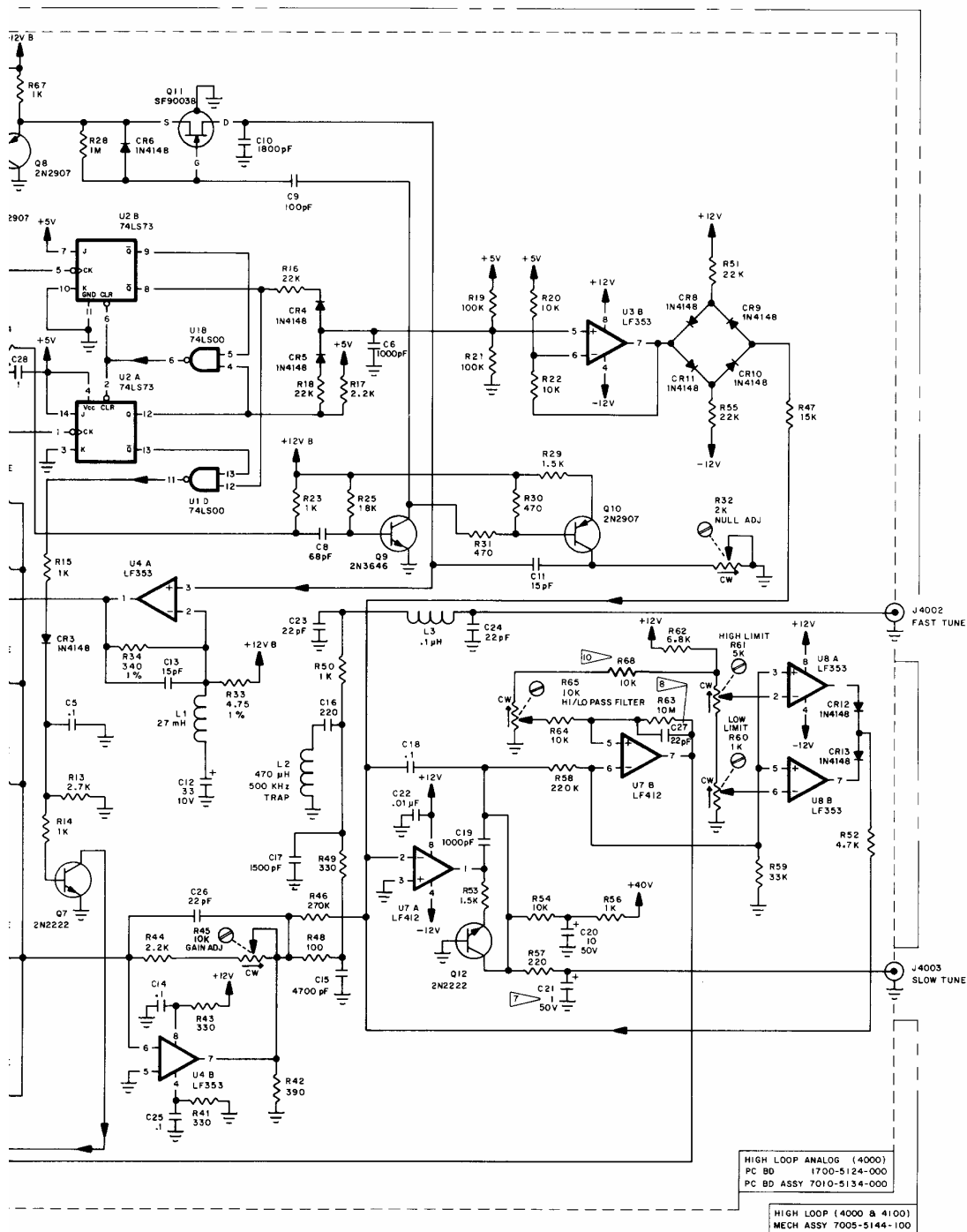
Figure 10-14a High Loop Module Circuit Schematic (Sheet 2 of 2)
