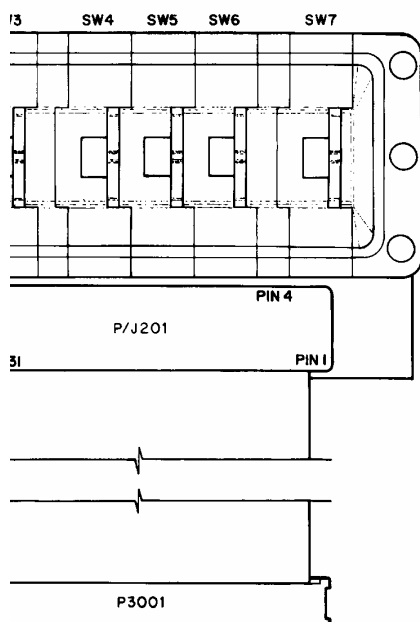
RF Thumbwheel Switch PC Board Assembly (200)
