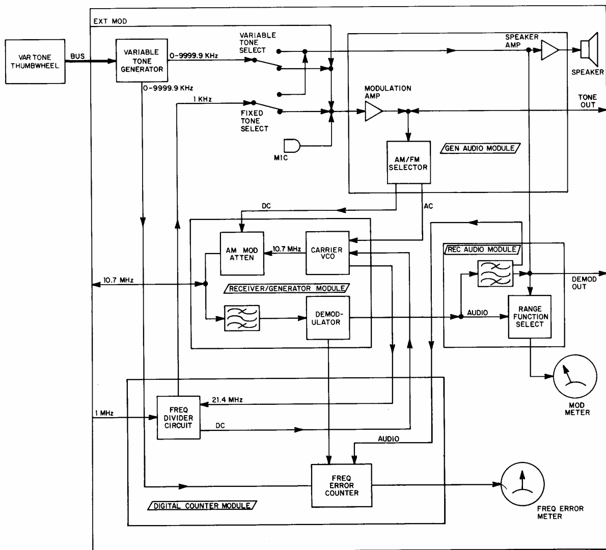
Figure 2-5 Audio System Block Diagram
