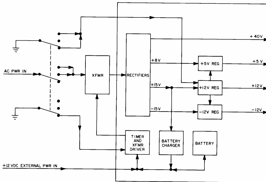
Figure 7-1 Power Supply Block Diagram
