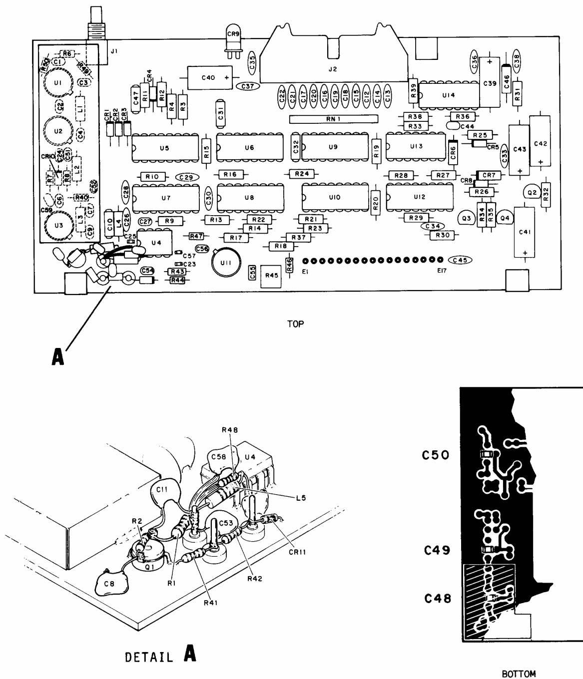
Figure 9-12 High Loop Divider PC Board Assembly (4100) (Thru SN 3074)
