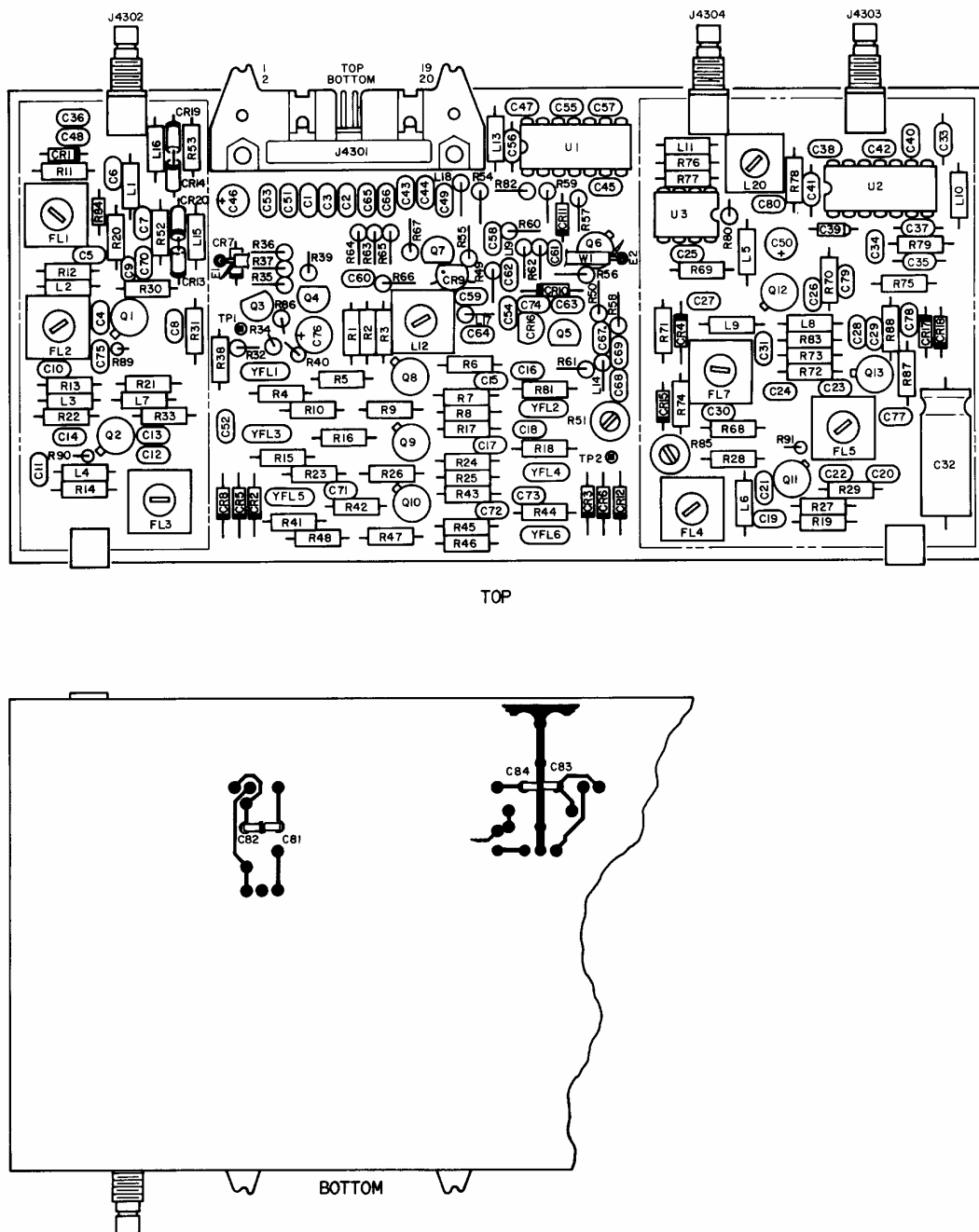
Figure 9-14 Receiver/Generator PC Board Assembly (4300)
