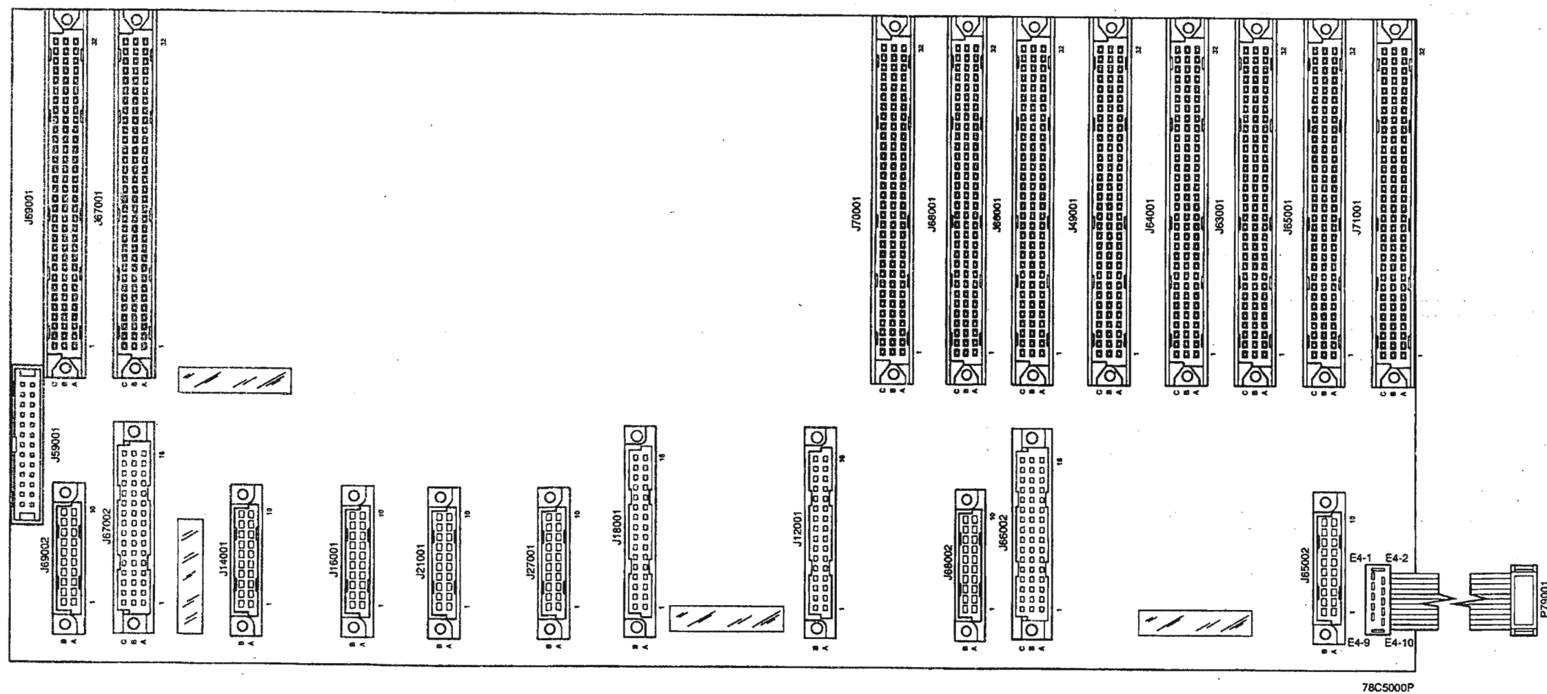
MOTHERBOARD PC BOARD ASSEMBLY (7010-7835-003C-F5)
