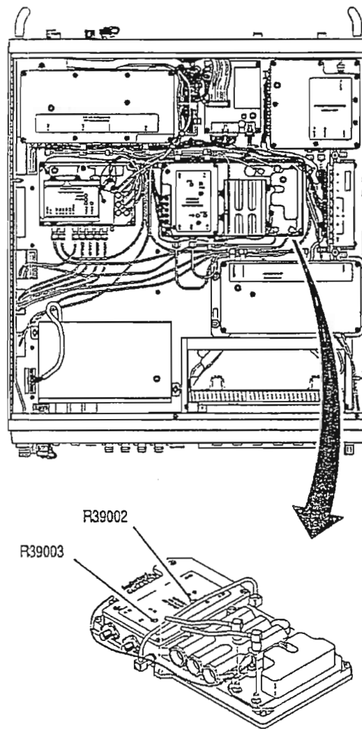
Figure 3-12 Receive IF Assembly Calibration Adjustments
