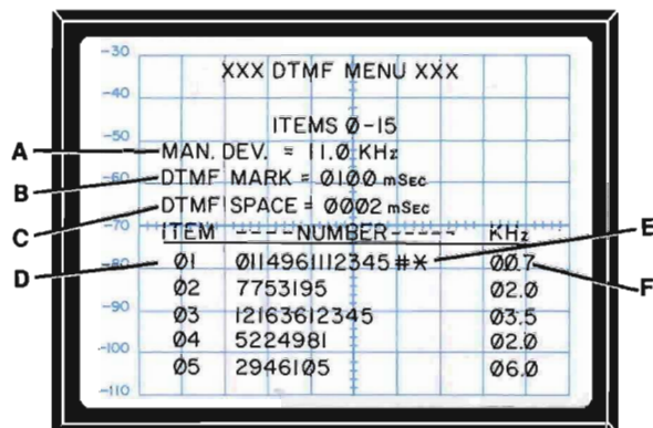
Figure 5-5 DTMF Menu
