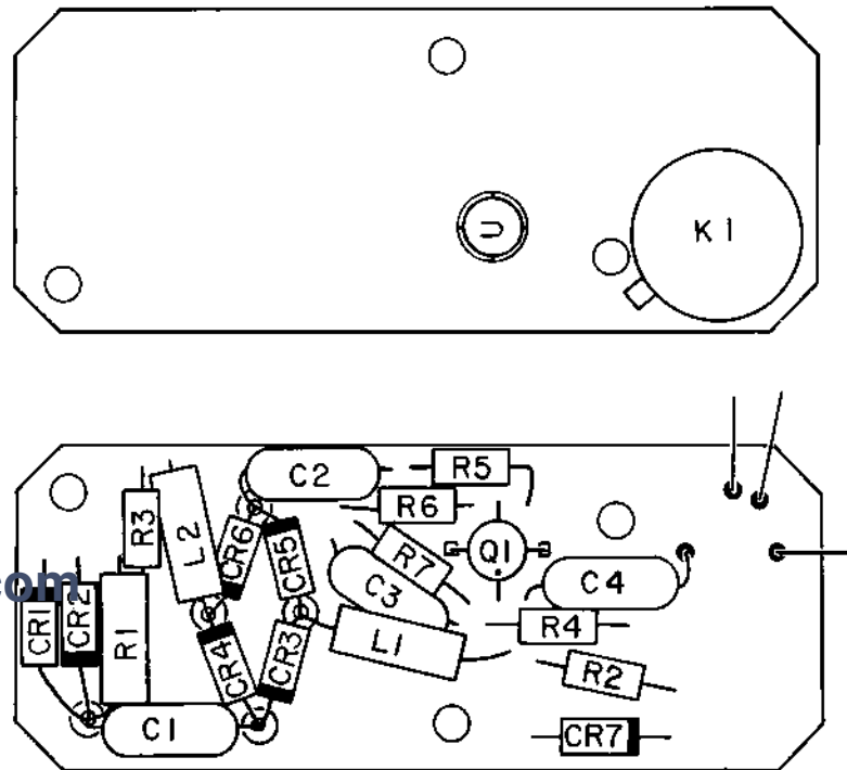
FIGURE 7-47 IF VOLTAGE PROTECT PC BOARD ASSEMBLY
