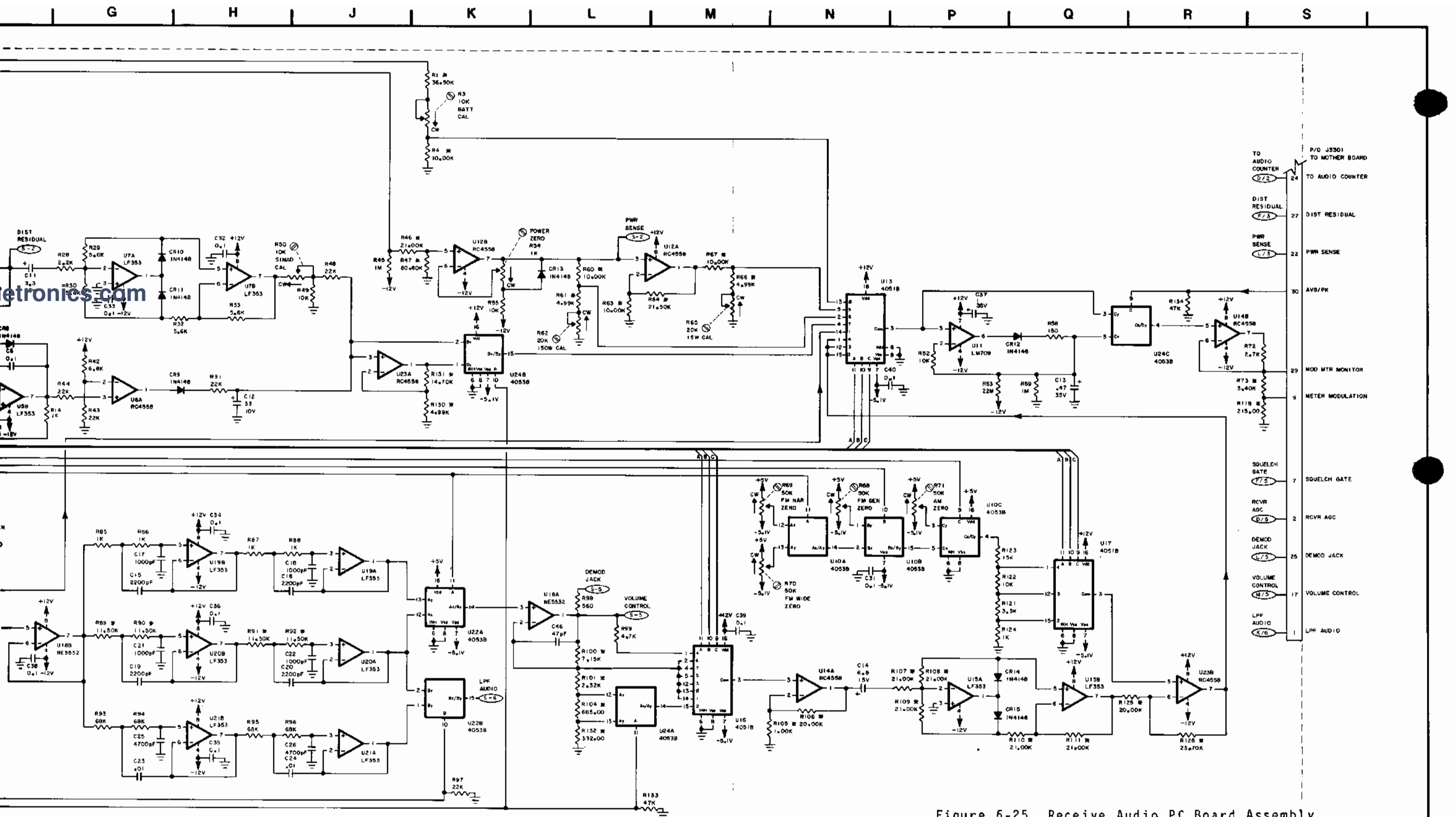
Figure 6-25 Receive Audio PC Board Assembly (0000-5213-301-F2)
