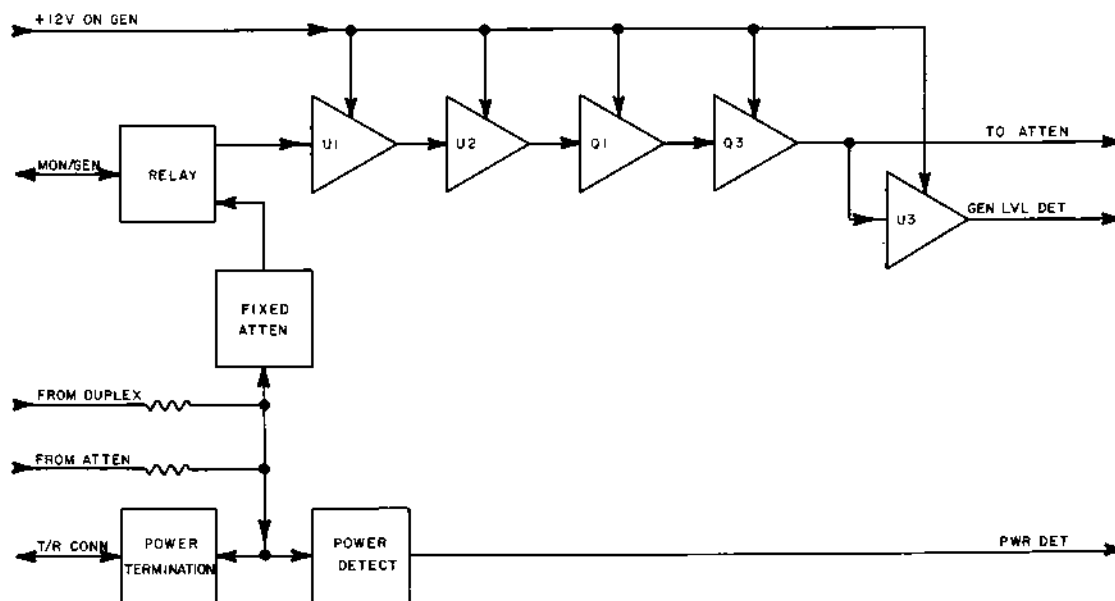
Figure 2-22 Output Amplifier Module Block Diagram
