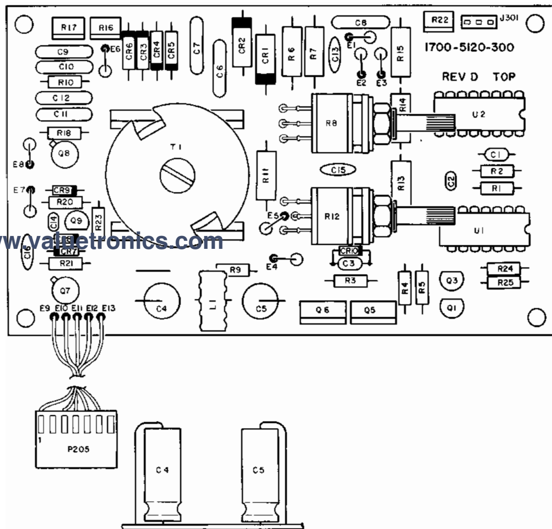
Scope Power PC Board (Rev D-9)
