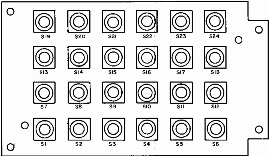
Keyboard PC Board (Rev A-5)
