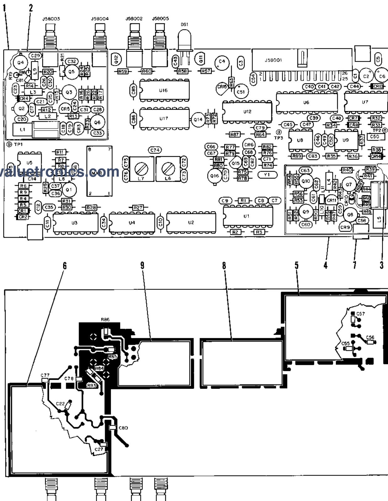
FIGURE 7-27A FAST LOW LOOP PC BOARD ASSEMBLY
