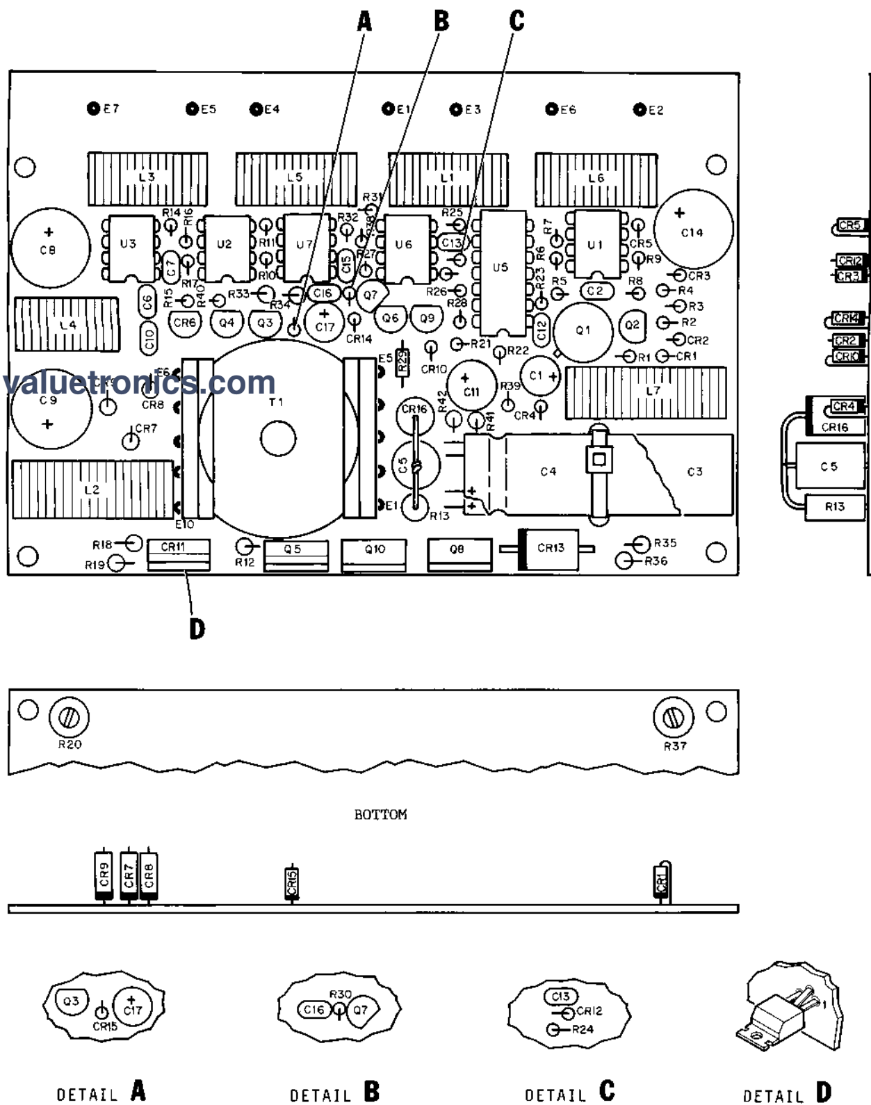
FIGURE 7-57A INVERTER SUPPLY PC BOARD ASSEMBLY
