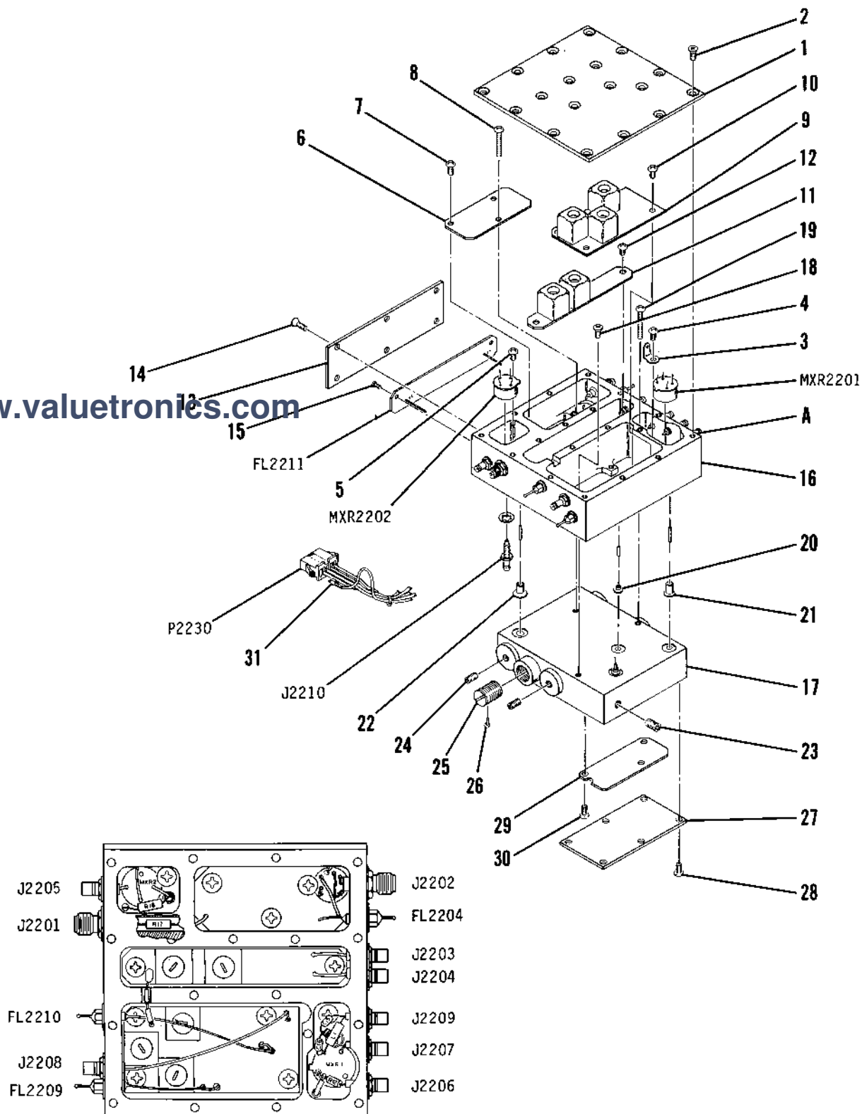
FIGURE 7-46 IF ASSEMBLY
