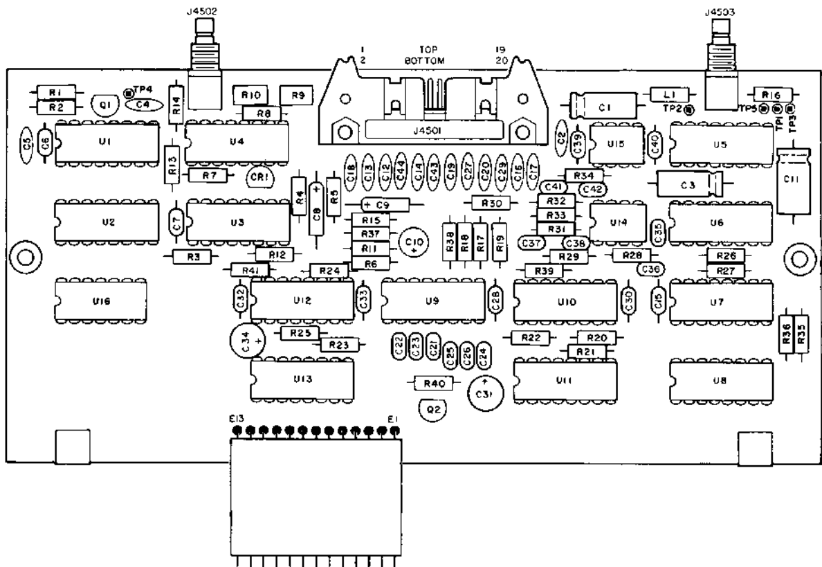
Digital Reference PC Board (Rev F-3)
