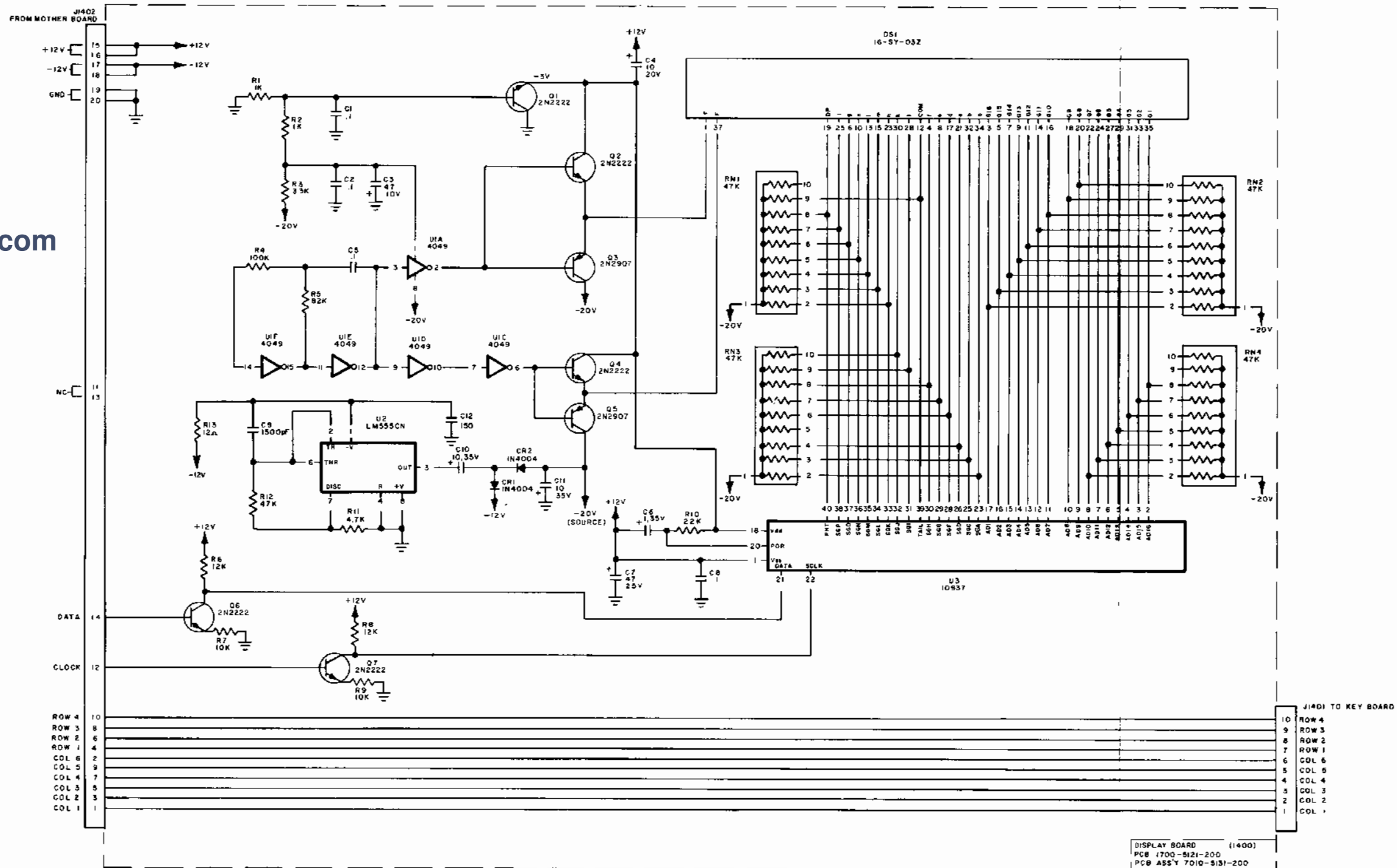
Figure 6-32 Display PC Board Assembly (0000-5111-200-E2)
