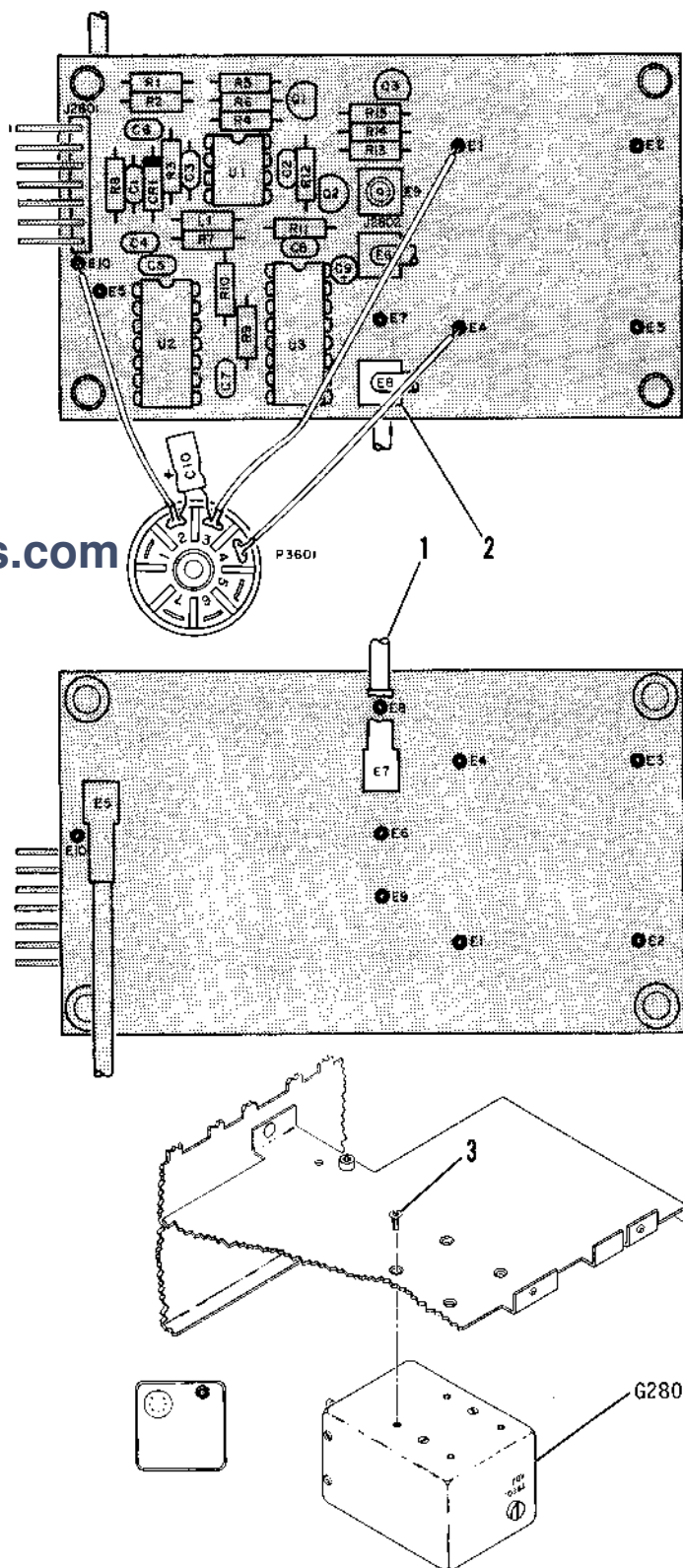
FIGURE 7-9 FREQUENCY STANDARD PC BOARD ASSEMBLY WITH .05 PPM OSCILLATOR (OPTION -02)
