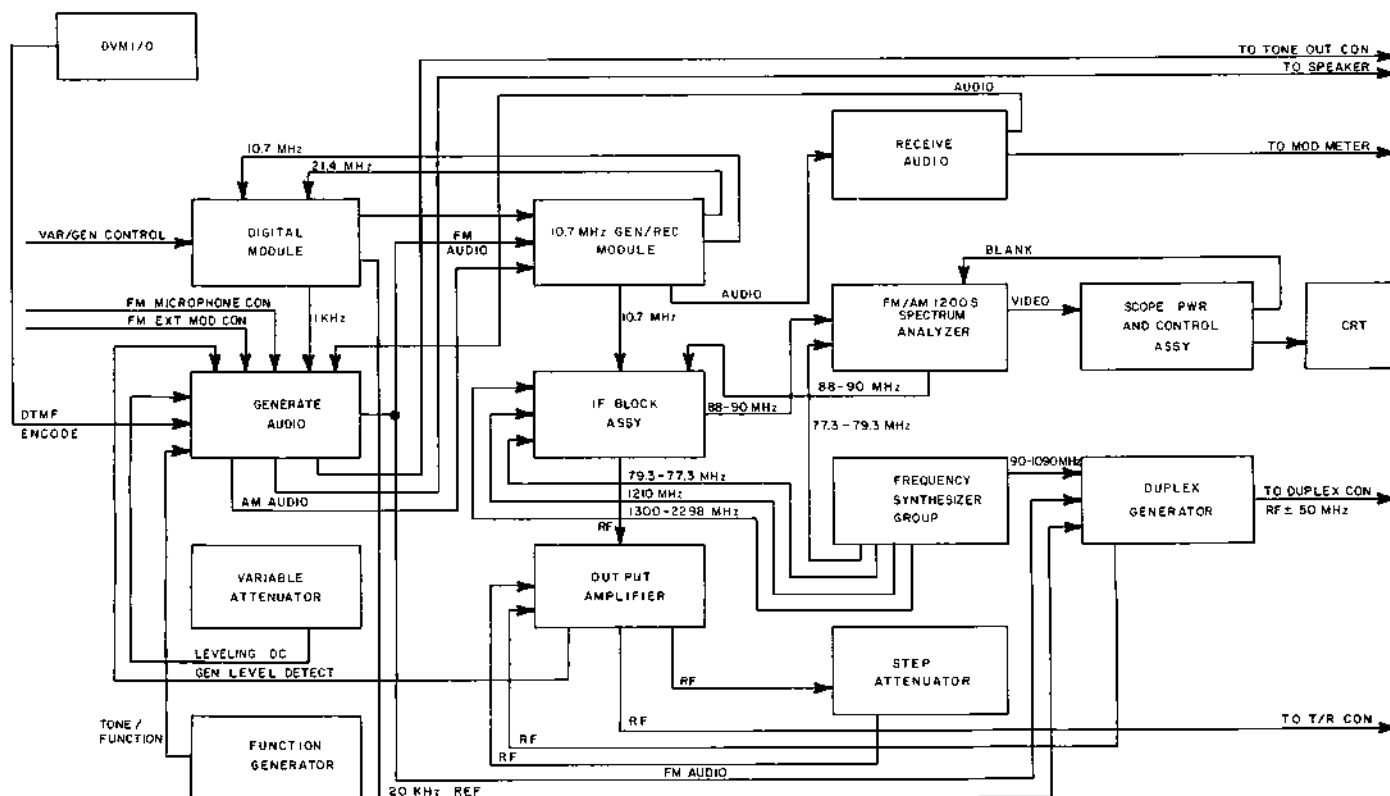
Figure 2-4 Generator Functional Block Diagram
