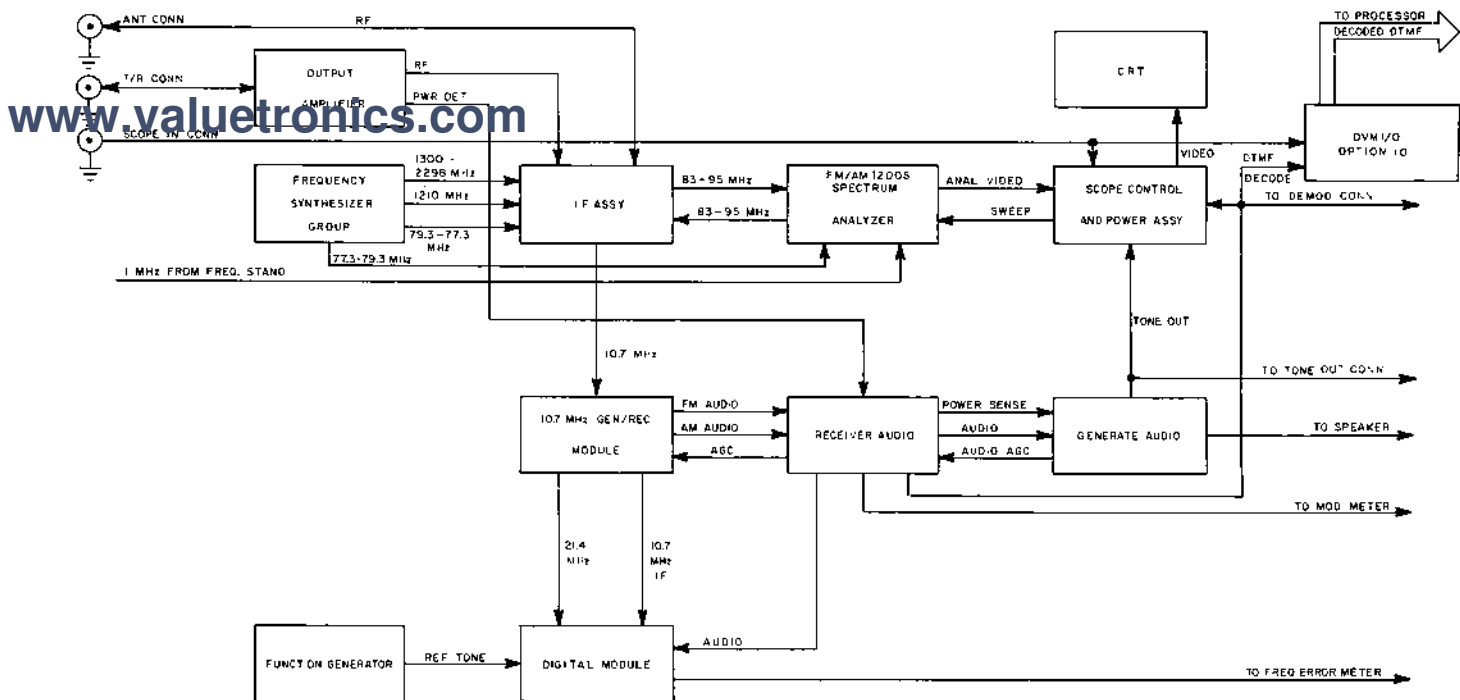
Figure 2-3 Receiver Functional Block Diagram
