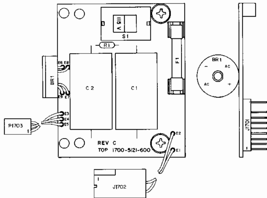
Line Supply PC Board Assembly (Rev D)
