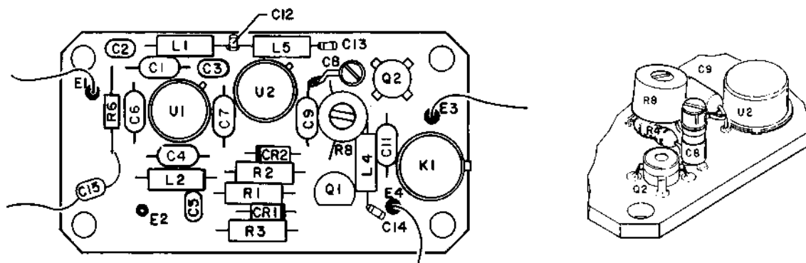
FIGURE 7-4 GENERATE AMP PC BOARD ASSEMBLY
