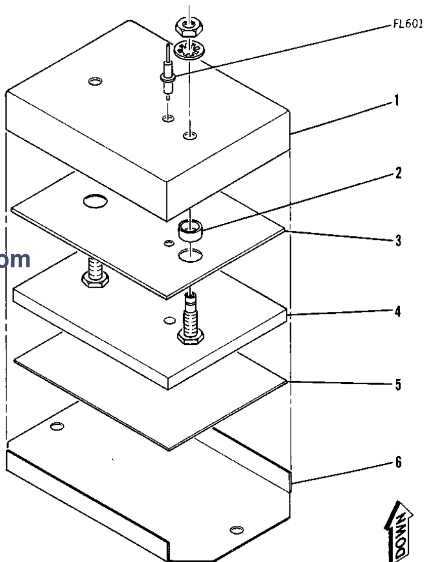
FIGURE 7-43 HIGH-LOW PASS FILTER ASSEMBLY
