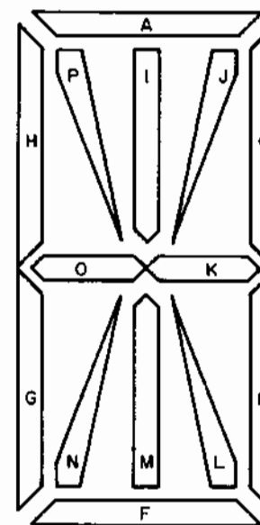
VFD DISPLAY WITH SEGMENT LOCATIONS IDENTIFIED (A THRU P)
