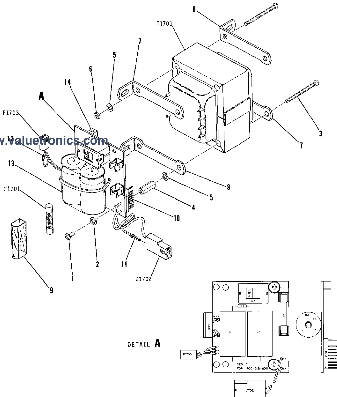
FIGURE 7-52 LINE SUPPLY PC BOARD ASSEMBLY
