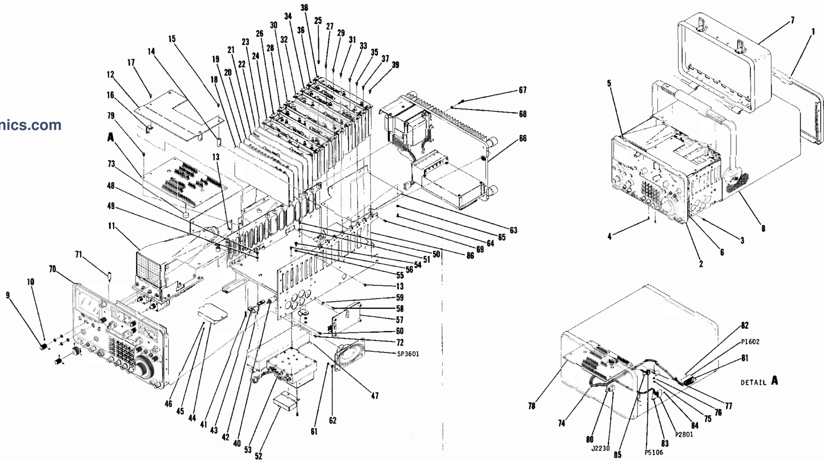
FIGURE 7-13 COMPOSITE ASSEMBLY
