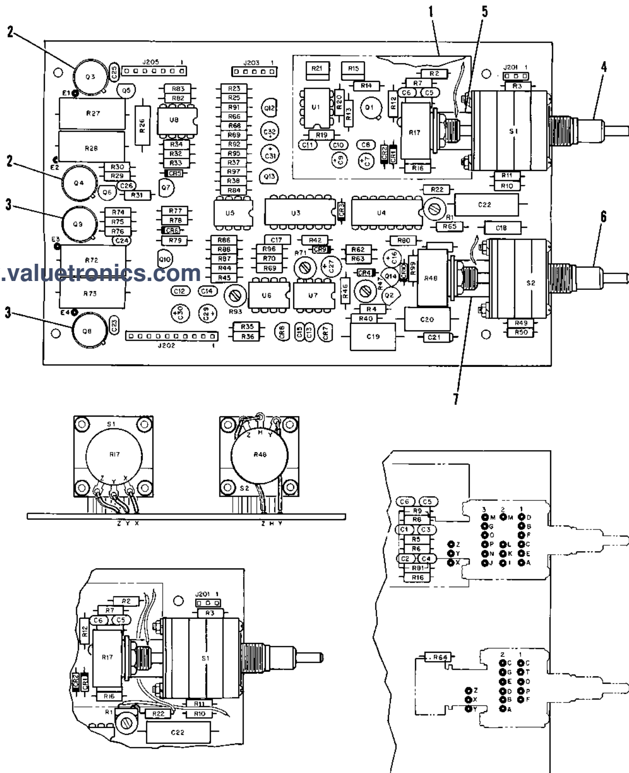
FIGURE 7-19 SCOPE CONTROL PC BOARD ASSEMBLY
