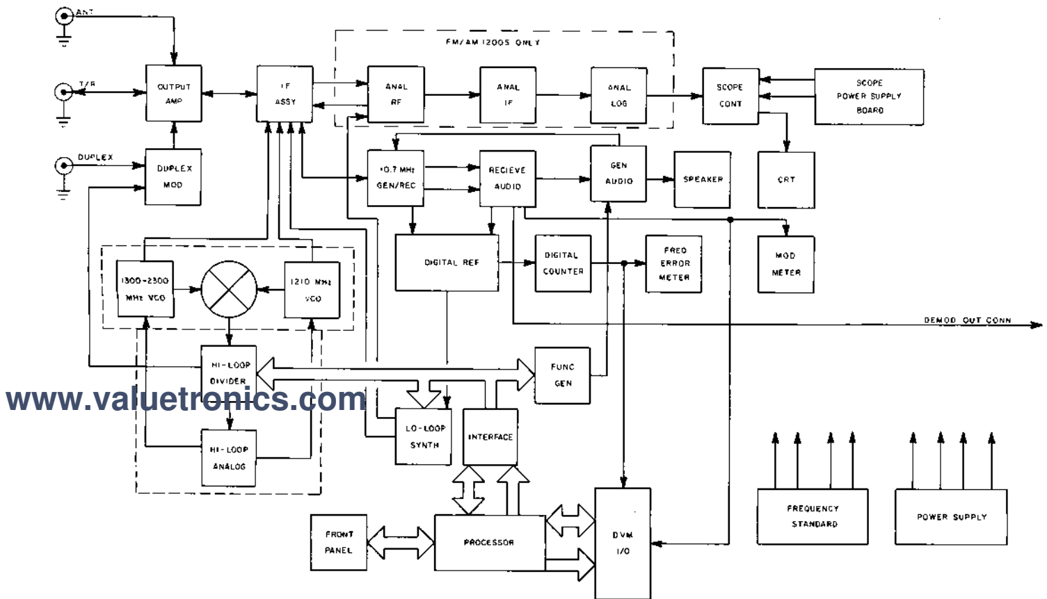
Figure 2-1 System Block Diagram
