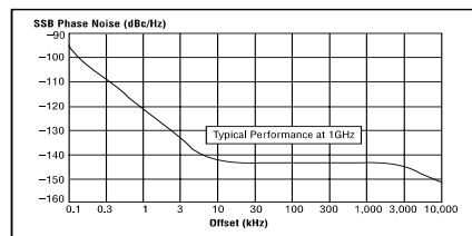
Typical phase noise performance at 1 GHz
