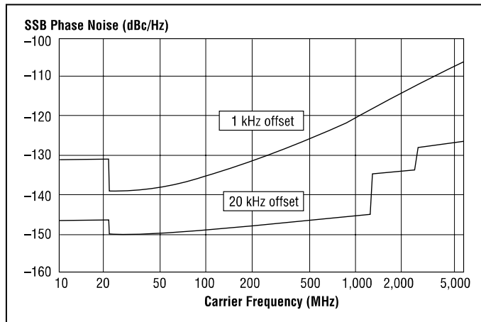
Typical Phase Noise Variation with Frequency
