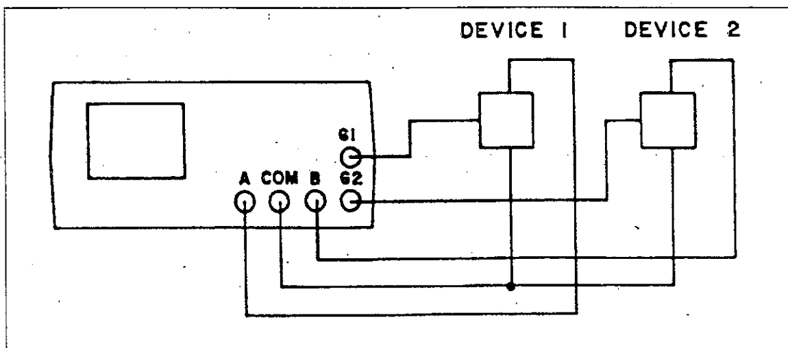
Figure 10-22. Pulse Generator Comparison Mode.
