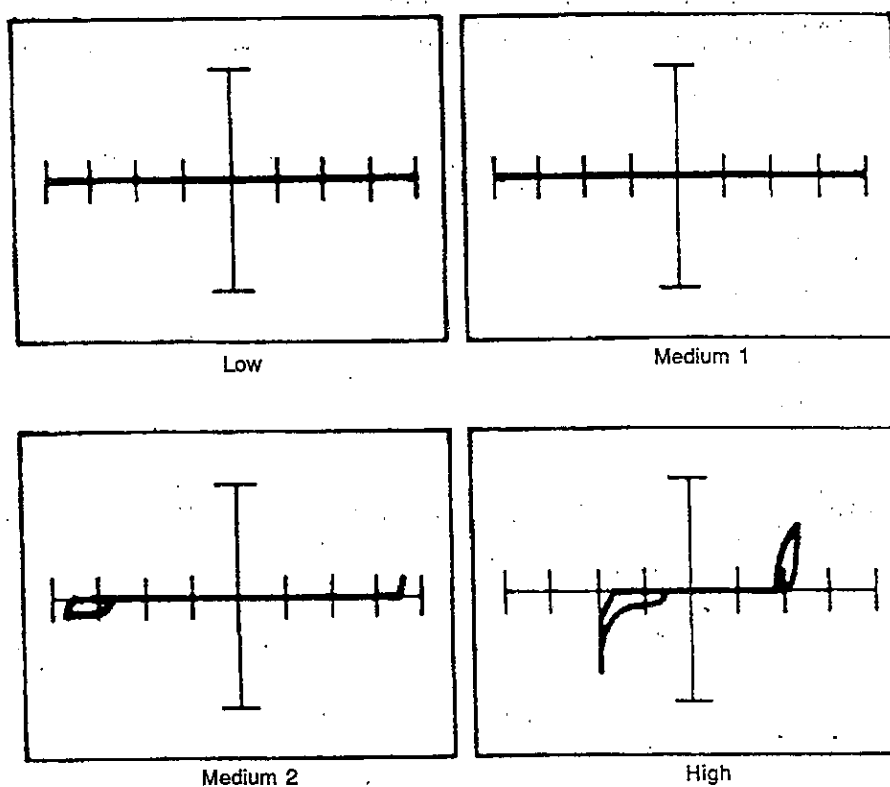
Figure 12-54. Signatures Between the WE Pin and the Ground Pin of a 2114A Static RAM at 60 Hz.
