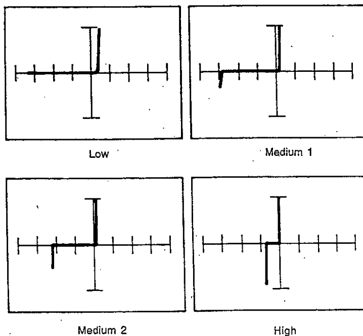
Figure 10-18. Signatures of the Base-Emitter of a 4N25 at 60 Hz. Pin 6 with Pin 4 as Common.
