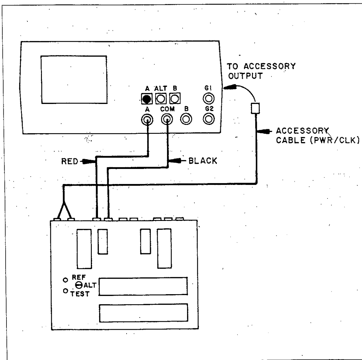
Figure 2-8. 2000/Switcher Interconnection.
