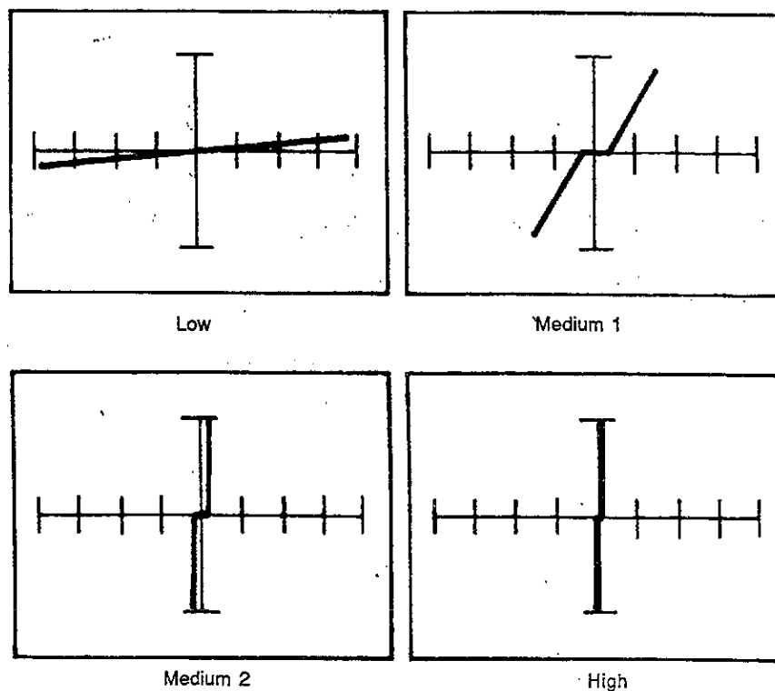
Figure 12-49. Signatures Between a Control Pin and V_{ss} - V_{dd} of a 4016B at 60 Hz.
