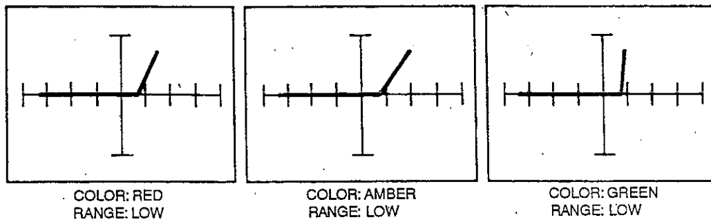
Figure 8-19. LED Signatures.
