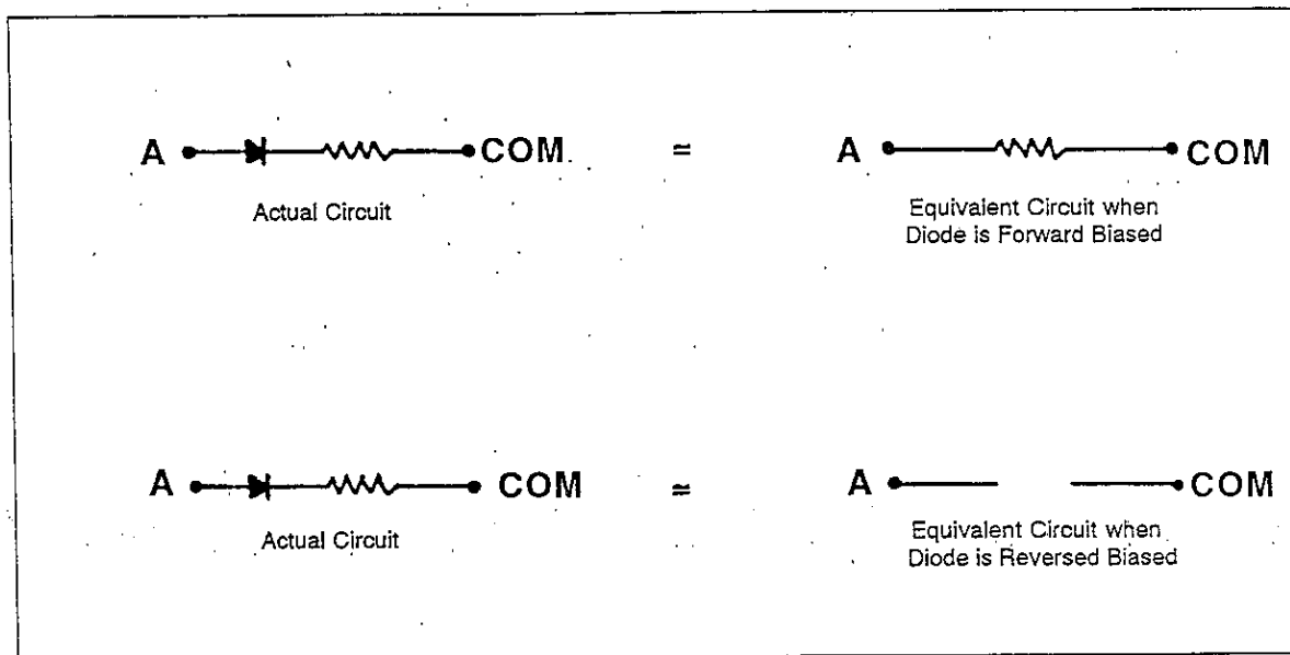
Figure 11-3. Diode/Resistor Equivalent Circuits.
