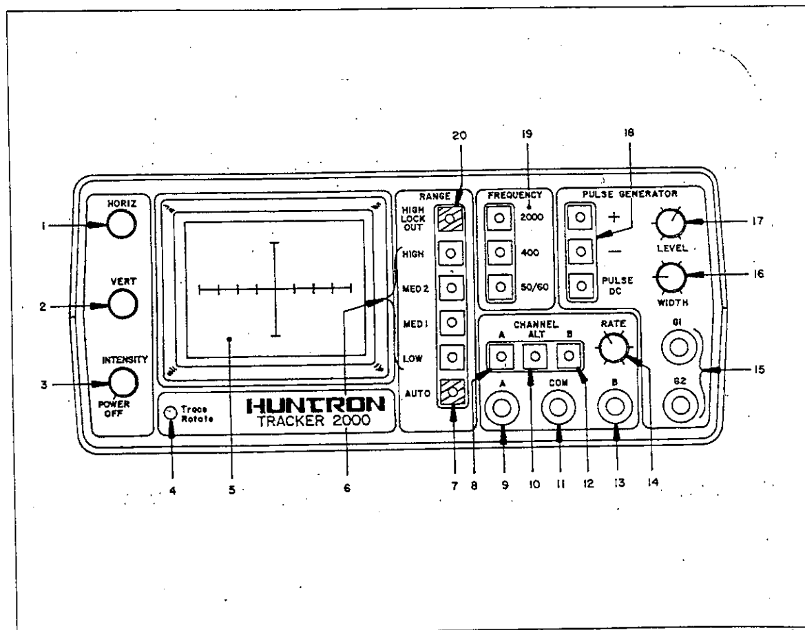
Figure 2-1. Front Panel.
