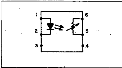
Figure 10-40. Pin Configuration of a CLM51 Photocell Optocoupler.
