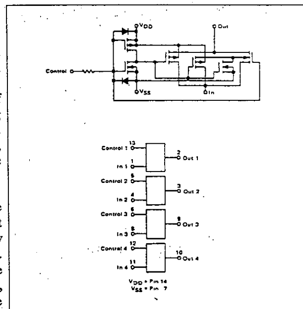
Figure 12-46. Schematic and Pin Layout of a 4016B.
