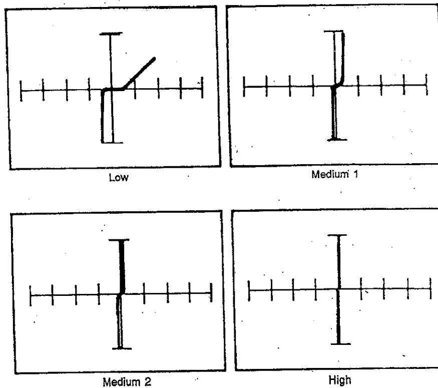
Figure 12-69. Signatures Between the Vcc Pin and the Ground Pin of a 6301-1J at 60 Hz.
