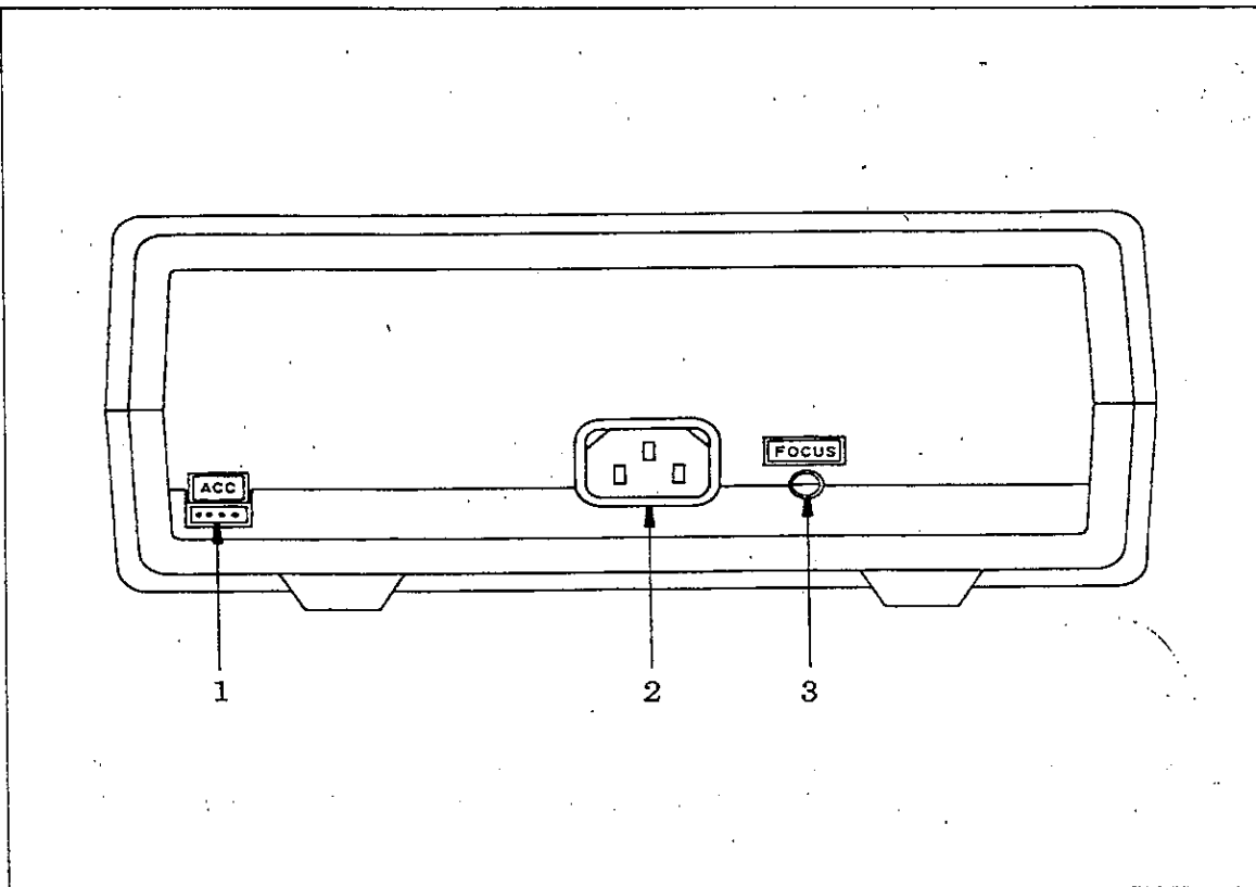
Figure 2-2. Back Panel.
